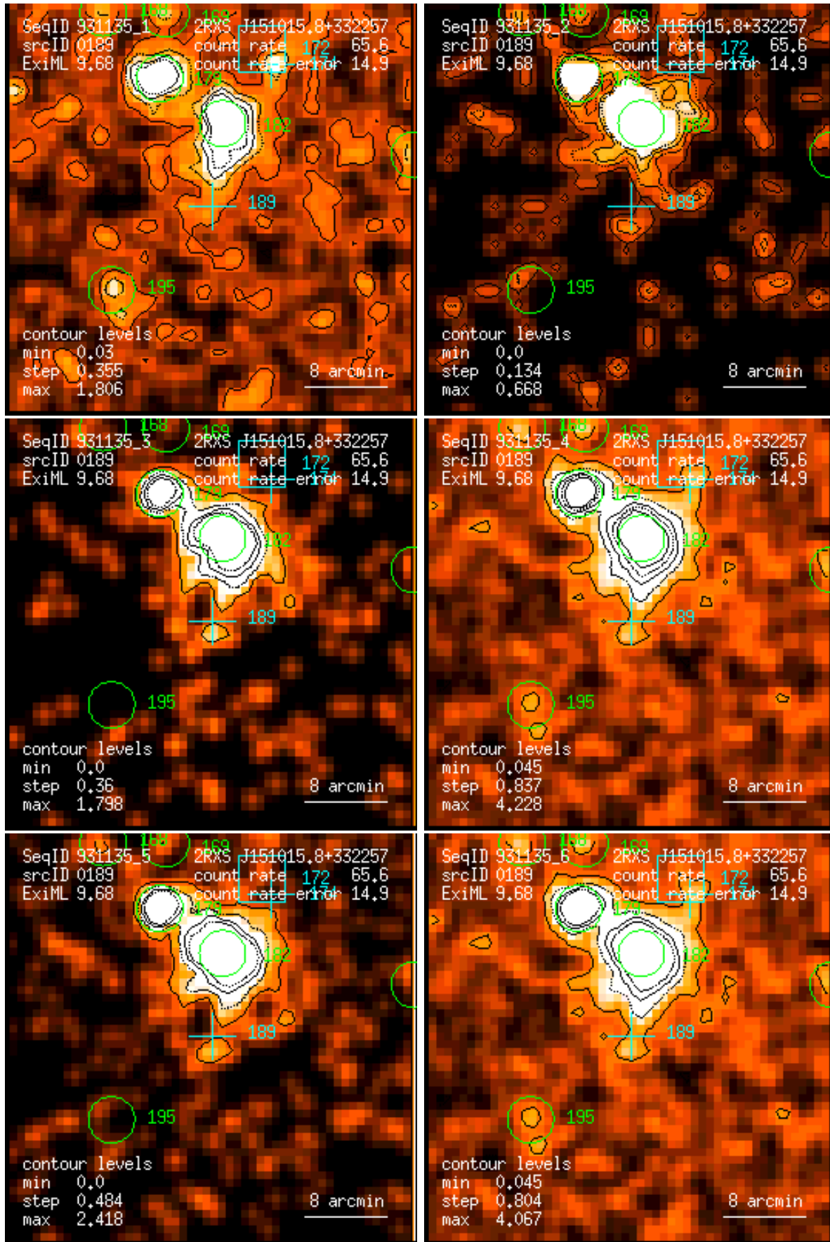
Figure 189: RASS 931135: detection 0189: band rate images, Gaussian filter: (1) PSPC channels 11 – 41, (2) 52 – 90, (3) 91 – 201, (4) 11 – 235, (5) 52 – 201, (6) 11 – 201. Broad band rates in counts/ks. Band rate contour levels in counts/ks/arcmin 2 .
