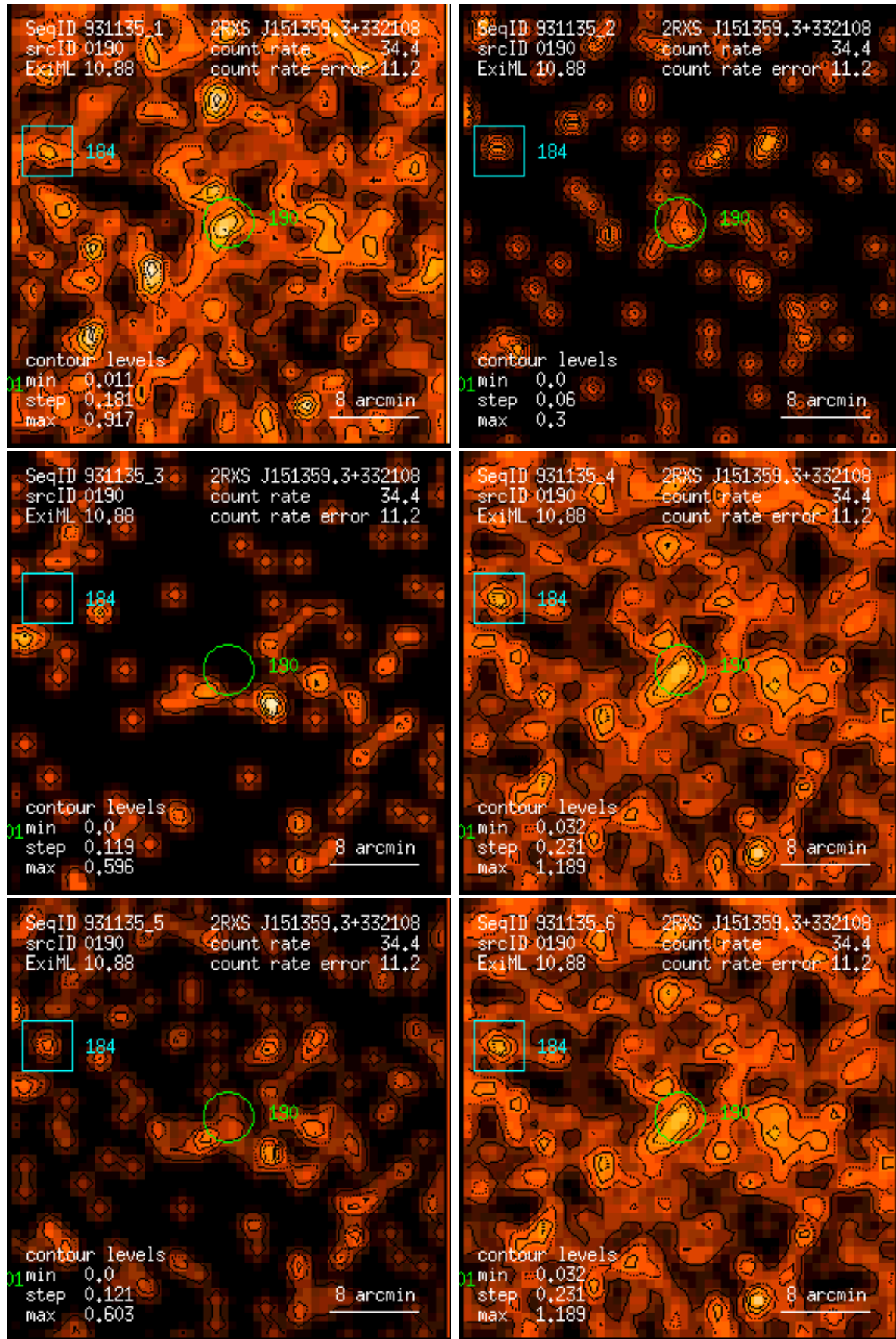
Figure 190: RASS 931135: detection 0190: band rate images, Gaussian filter: (1) PSPC channels 11 – 41, (2) 52 – 90, (3) 91 – 201, (4) 11 – 235, (5) 52 – 201, (6) 11 – 201. Broad band rates in counts/ks. Band rate contour levels in counts/ks/arcmin 2 .
