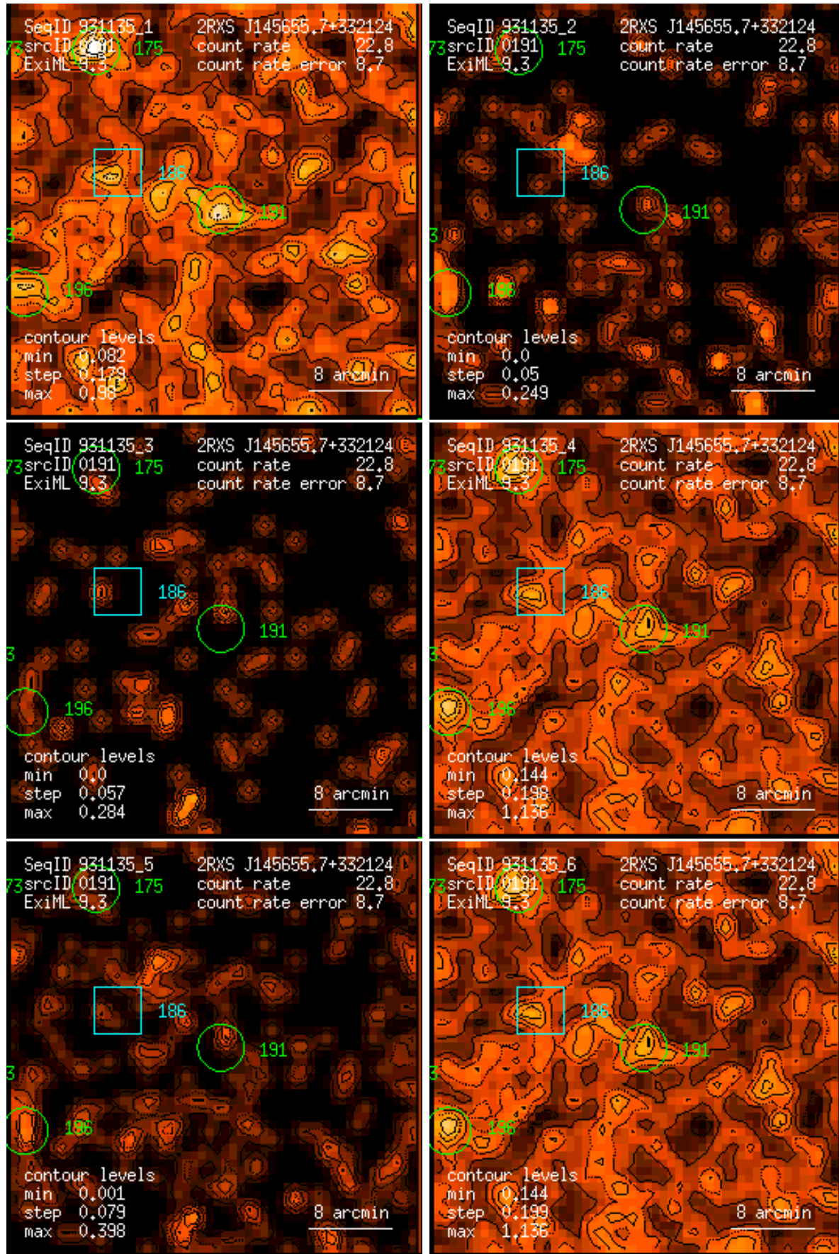
Figure 191: RASS 931135: detection 0191: band rate images, Gaussian filter: (1) PSPC channels 11 – 41, (2) 52 – 90, (3) 91 – 201, (4) 11 – 235, (5) 52 – 201, (6) 11 – 201. Broad band rates in counts/ks. Band rate contour levels in counts/ks/arcmin 2 .
