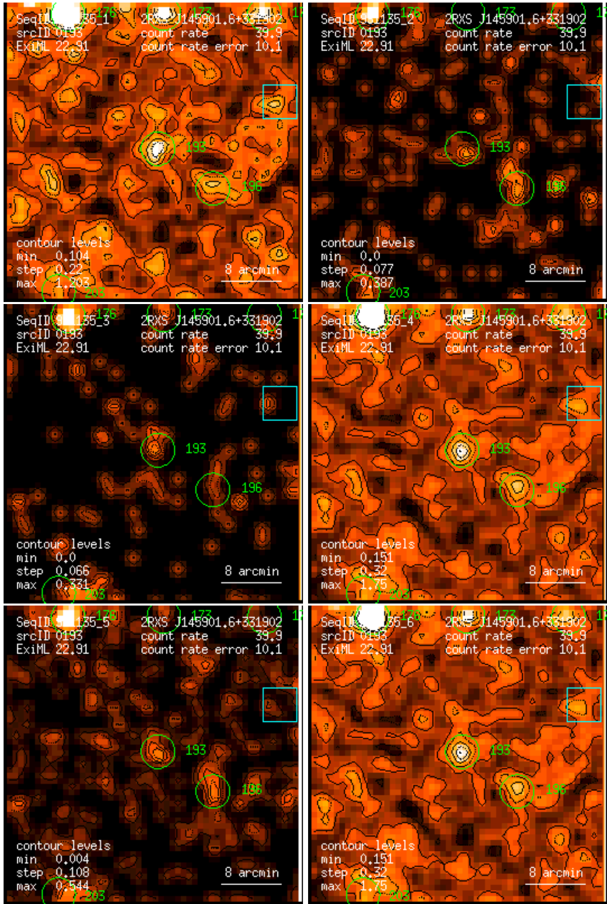
Figure 193: RASS 931135: detection 0193: band rate images, Gaussian filter: (1) PSPC channels 11 – 41, (2) 52 – 90, (3) 91 – 201, (4) 11 – 235, (5) 52 – 201, (6) 11 – 201. Broad band rates in counts/ks. Band rate contour levels in counts/ks/arcmin 2 .
