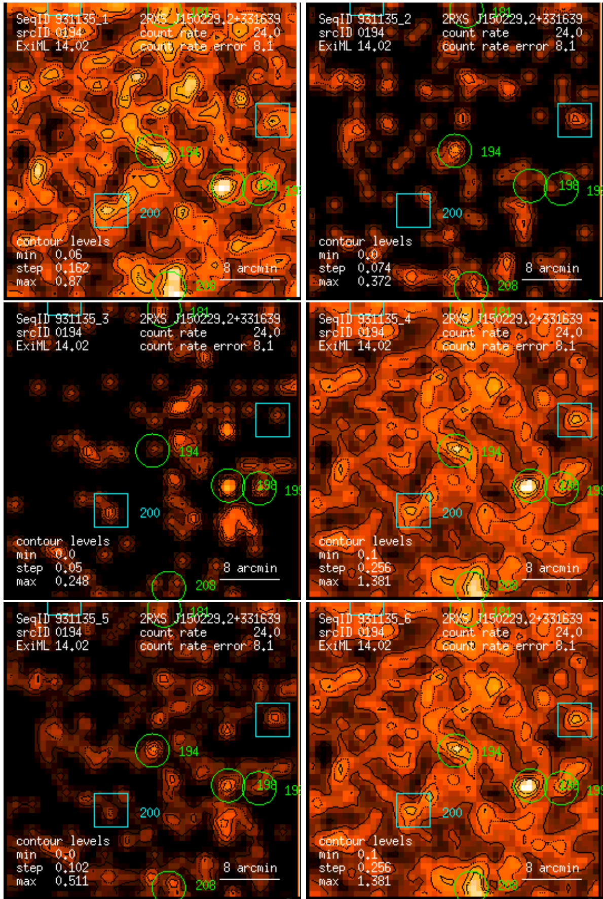
Figure 194: RASS 931135: detection 0194: band rate images, Gaussian filter: (1) PSPC channels 11 – 41, (2) 52 – 90, (3) 91 – 201, (4) 11 – 235, (5) 52 – 201, (6) 11 – 201. Broad band rates in counts/ks. Band rate contour levels in counts/ks/arcmin 2 .
