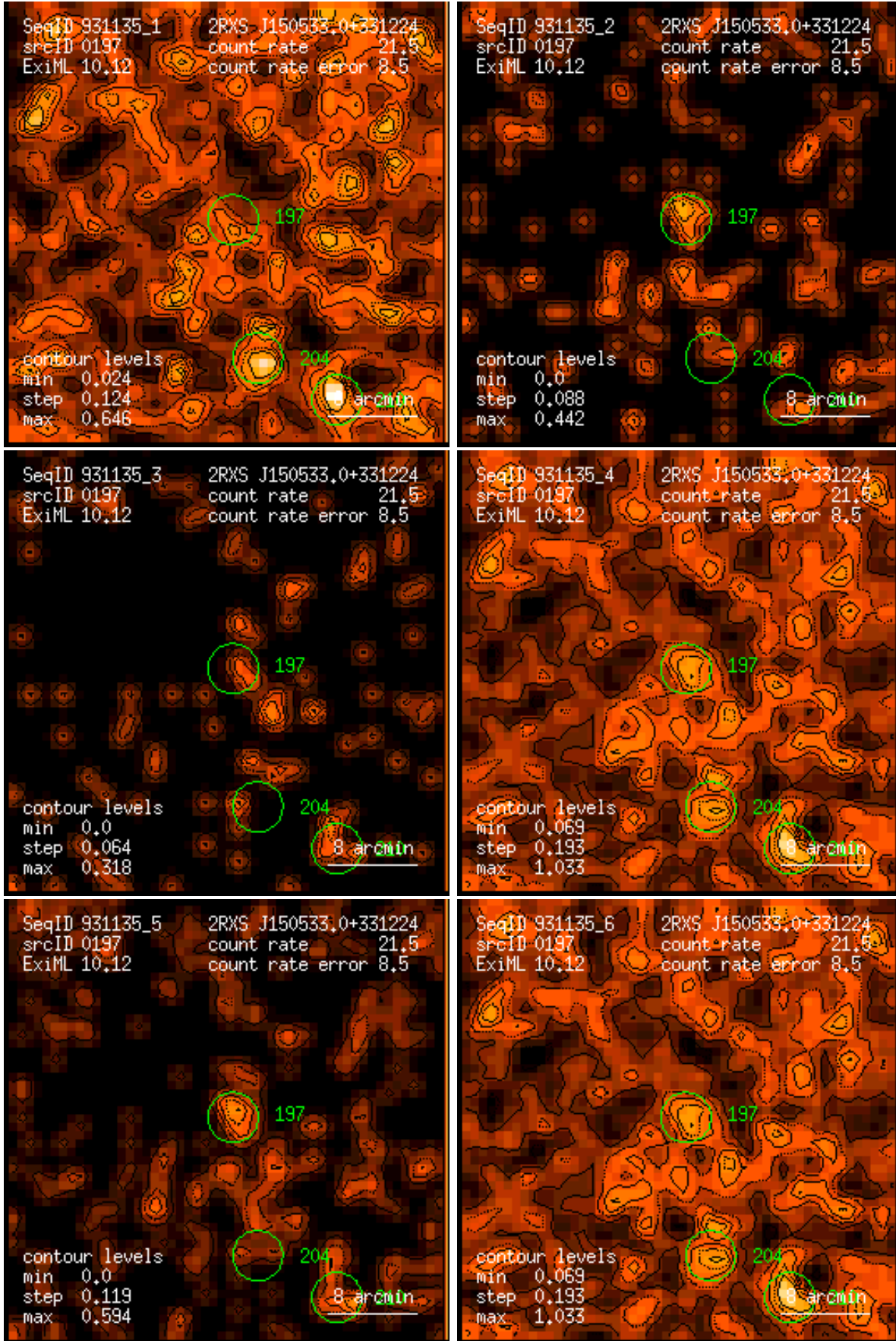
Figure 197: RASS 931135: detection 0197: band rate images, Gaussian filter: (1) PSPC channels 11 – 41, (2) 52 – 90, (3) 91 – 201, (4) 11 – 235, (5) 52 – 201, (6) 11 – 201. Broad band rates in counts/ks. Band rate contour levels in counts/ks/arcmin 2 .
