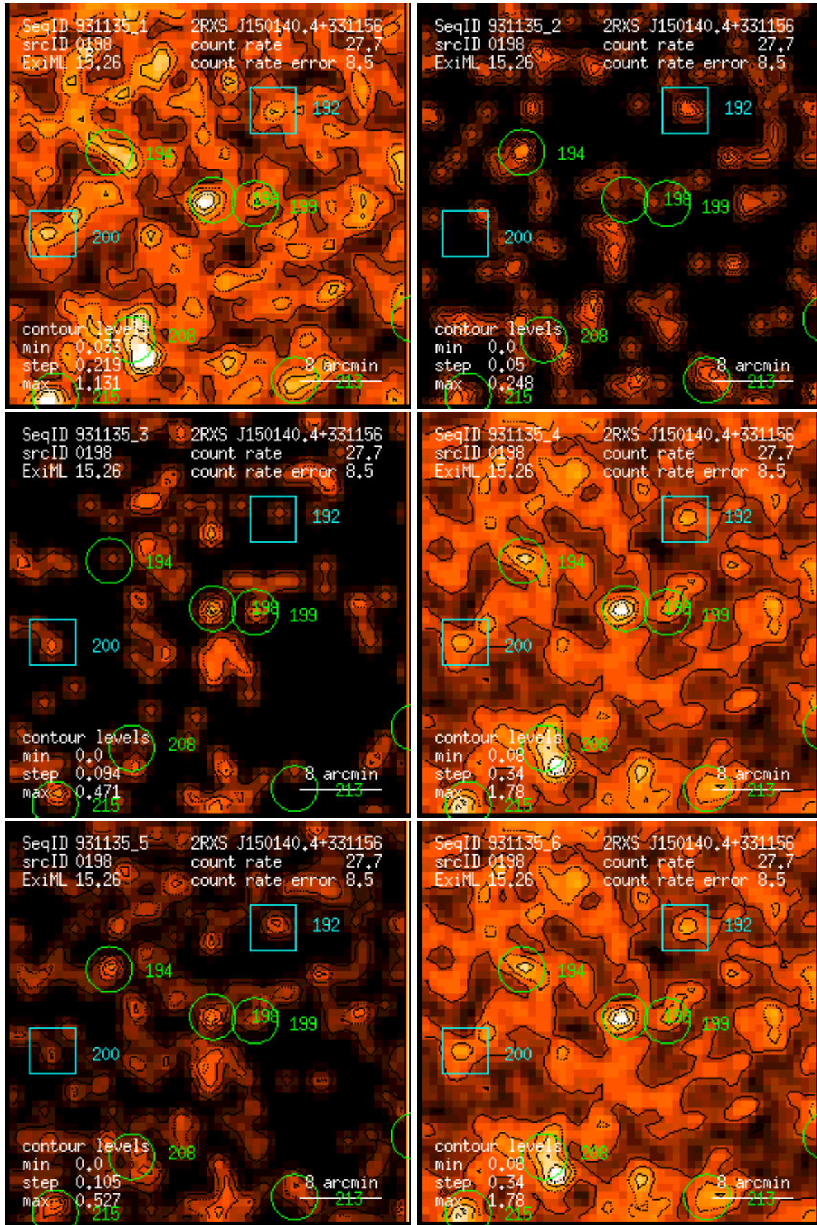
Figure 198: RASS 931135: detection 0198: band rate images, Gaussian filter: (1) PSPC channels 11 – 41, (2) 52 – 90, (3) 91 – 201, (4) 11 – 235, (5) 52 – 201, (6) 11 – 201. Broad band rates in counts/ks. Band rate contour levels in counts/ks/arcmin 2 .
