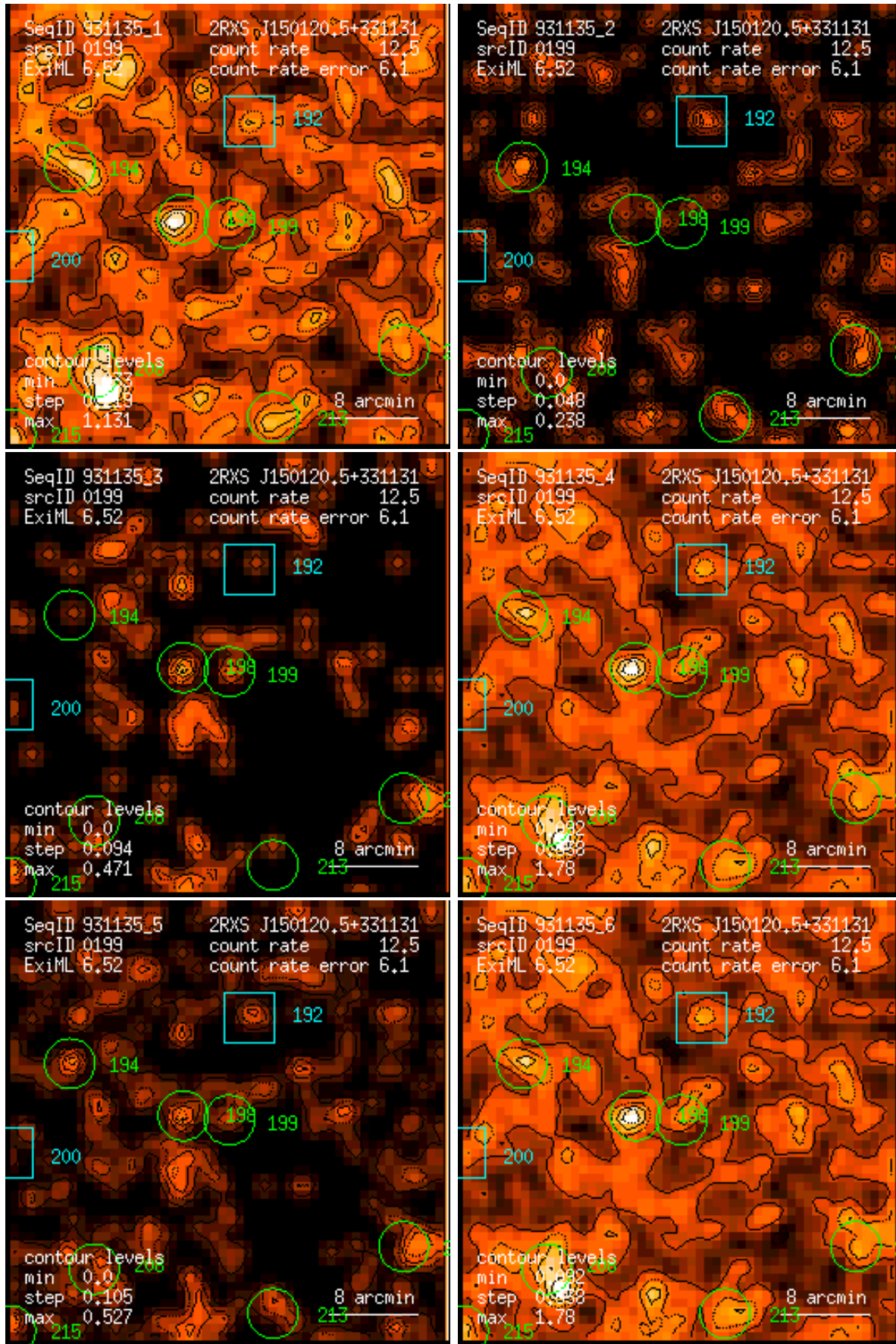
Figure 199: RASS 931135: detection 0199: band rate images, Gaussian filter: (1) PSPC channels 11 – 41, (2) 52 – 90, (3) 91 – 201, (4) 11 – 235, (5) 52 – 201, (6) 11 – 201. Broad band rates in counts/ks. Band rate contour levels in counts/ks/arcmin 2 .
