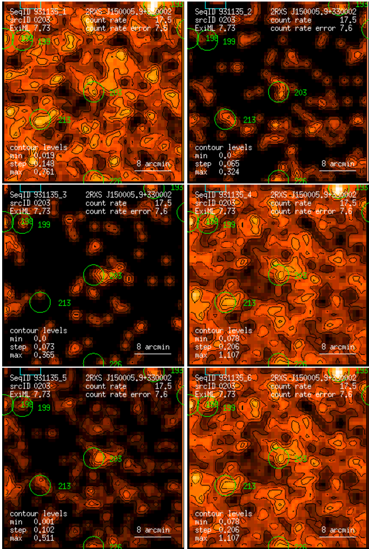
Figure 203: RASS 931135: detection 0203: band rate images, Gaussian filter: (1) PSPC channels 11 – 41, (2) 52 – 90, (3) 91 – 201, (4) 11 – 235, (5) 52 – 201, (6) 11 – 201. Broad band rates in counts/ks. Band rate contour levels in counts/ks/arcmin 2 .
