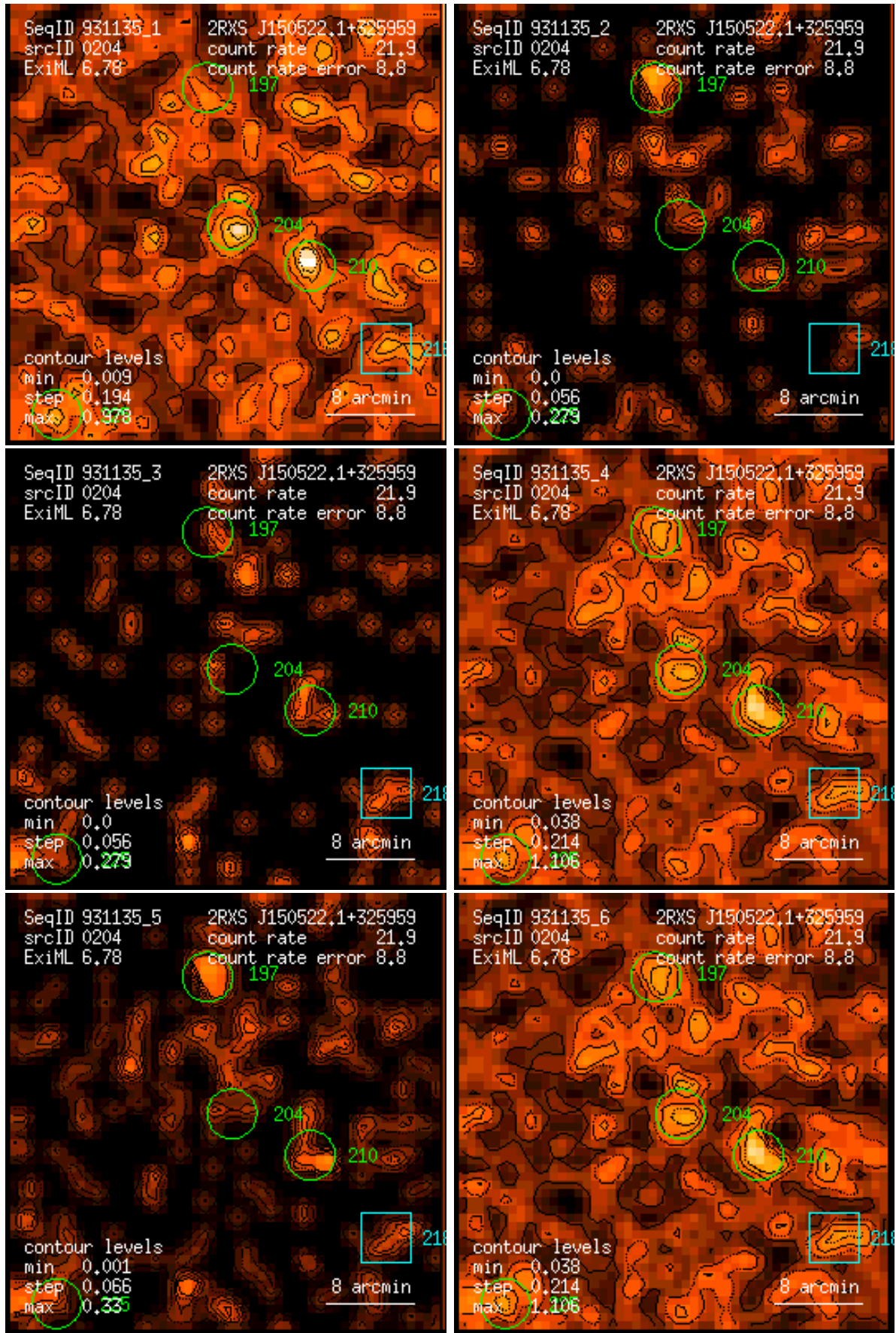
Figure 204: RASS 931135: detection 0204: band rate images, Gaussian filter: (1) PSPC channels 11 – 41, (2) 52 – 90, (3) 91 – 201, (4) 11 – 235, (5) 52 – 201, (6) 11 – 201. Broad band rates in counts/ks. Band rate contour levels in counts/ks/arcmin 2 .
