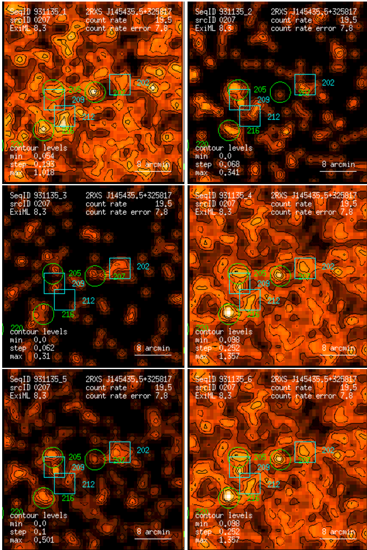
Figure 207: RASS 931135: detection 0207: band rate images, Gaussian filter: (1) PSPC channels 11 – 41, (2) 52 – 90, (3) 91 – 201, (4) 11 – 235, (5) 52 – 201, (6) 11 – 201. Broad band rates in counts/ks. Band rate contour levels in counts/ks/arcmin 2 .
