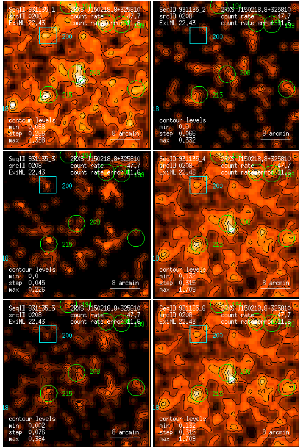
Figure 208: RASS 931135: detection 0208: band rate images, Gaussian filter: (1) PSPC channels 11 – 41, (2) 52 – 90, (3) 91 – 201, (4) 11 – 235, (5) 52 – 201, (6) 11 – 201. Broad band rates in counts/ks. Band rate contour levels in counts/ks/arcmin 2 .
