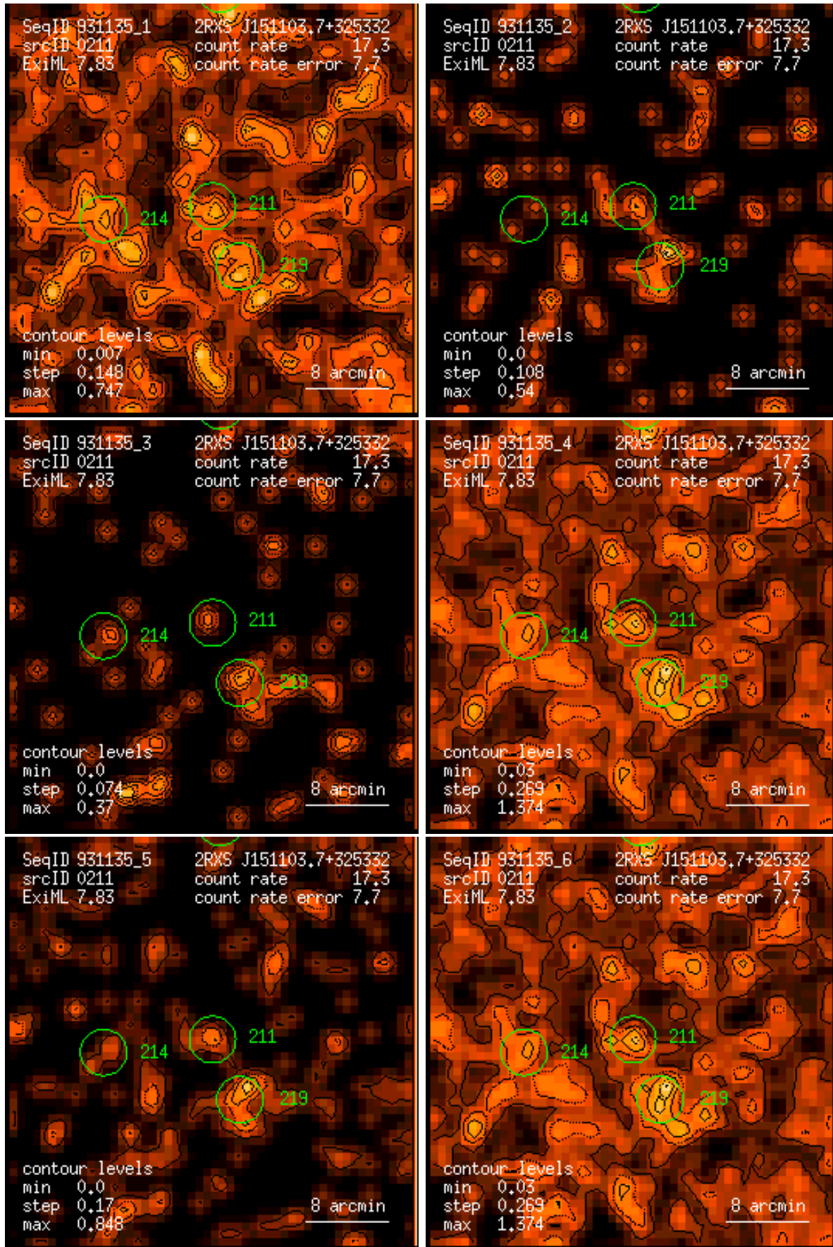
Figure 211: RASS 931135: detection 0211: band rate images, Gaussian filter: (1) PSPC channels 11 – 41, (2) 52 – 90, (3) 91 – 201, (4) 11 – 235, (5) 52 – 201, (6) 11 – 201. Broad band rates in counts/ks. Band rate contour levels in counts/ks/arcmin 2 .
