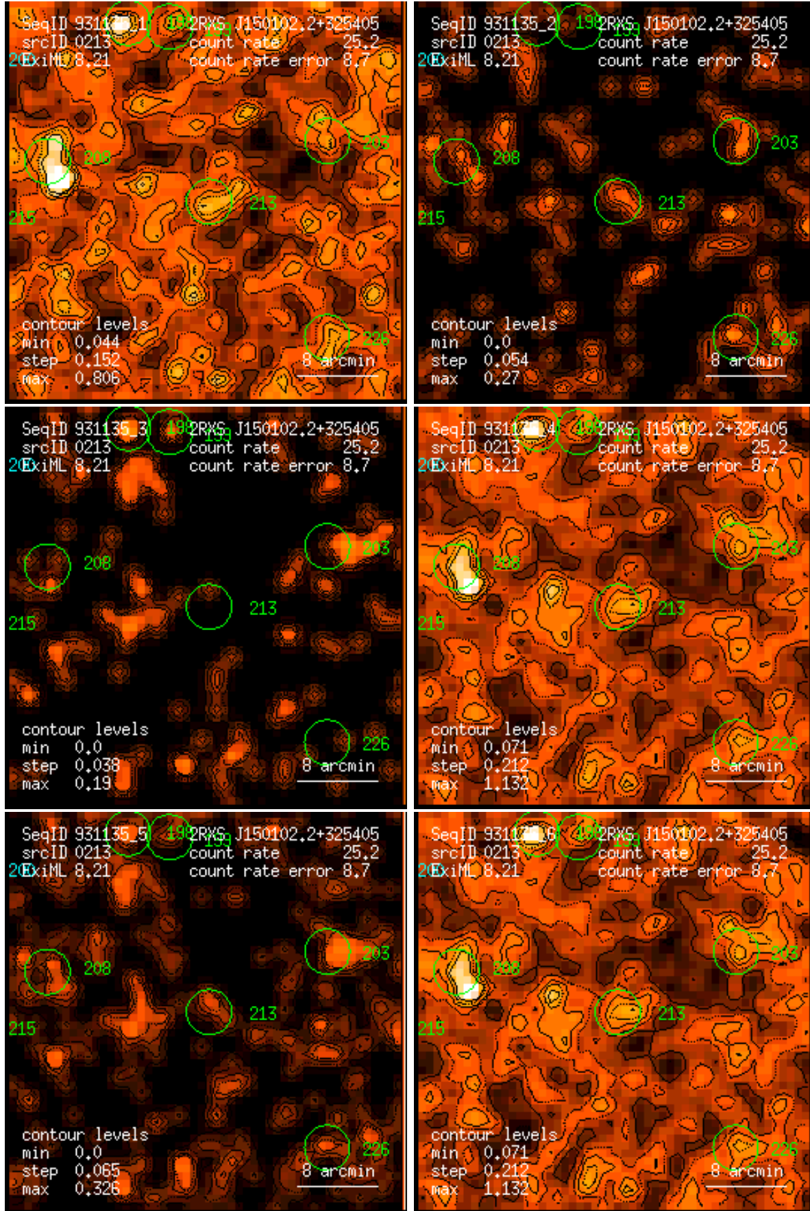
Figure 213: RASS 931135: detection 0213: band rate images, Gaussian filter: (1) PSPC channels 11 – 41, (2) 52 – 90, (3) 91 – 201, (4) 11 – 235, (5) 52 – 201, (6) 11 – 201. Broad band rates in counts/ks. Band rate contour levels in counts/ks/arcmin 2 .
