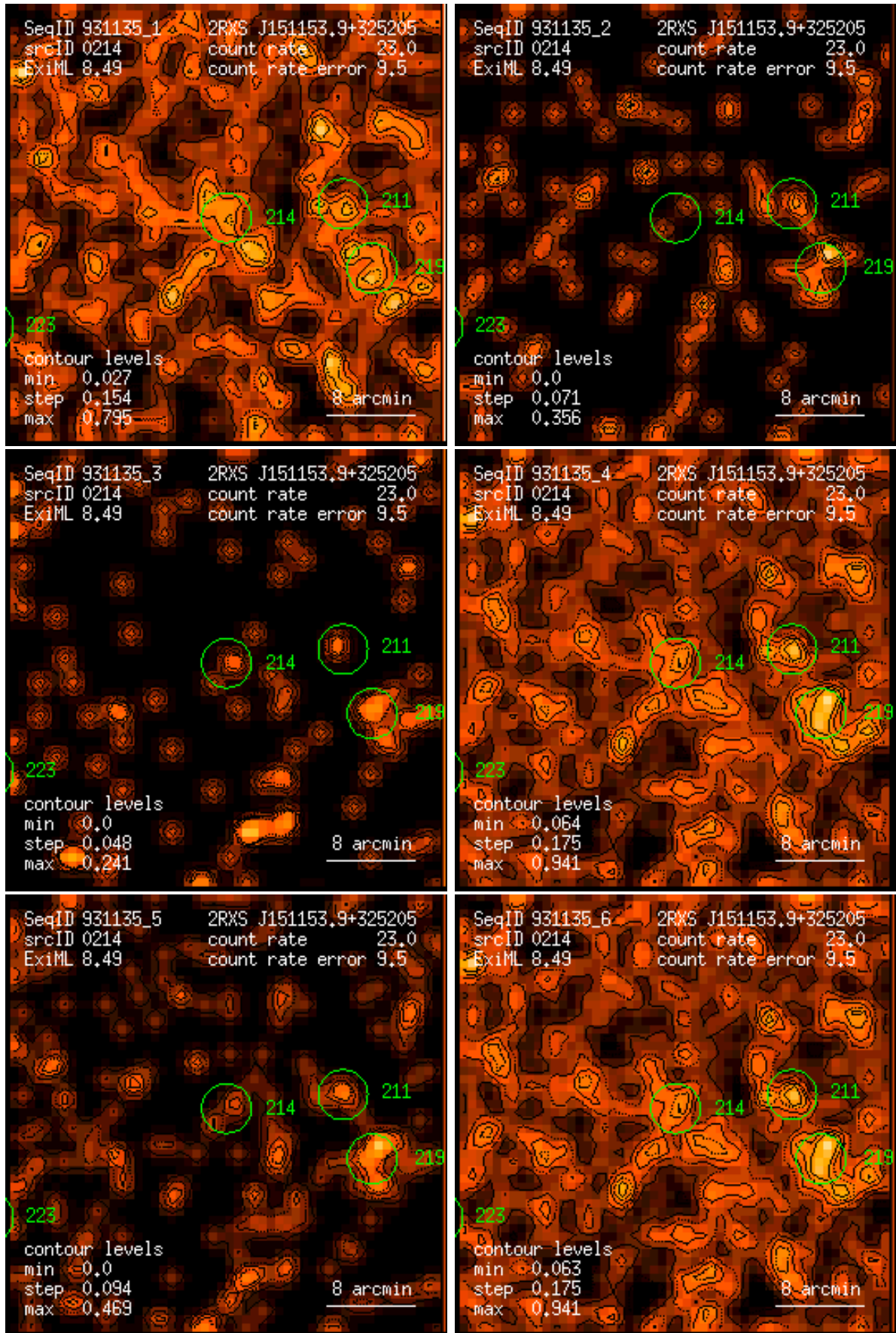
Figure 214: RASS 931135: detection 0214: band rate images, Gaussian filter: (1) PSPC channels 11 – 41, (2) 52 – 90, (3) 91 – 201, (4) 11 – 235, (5) 52 – 201, (6) 11 – 201. Broad band rates in counts/ks. Band rate contour levels in counts/ks/arcmin 2 .
