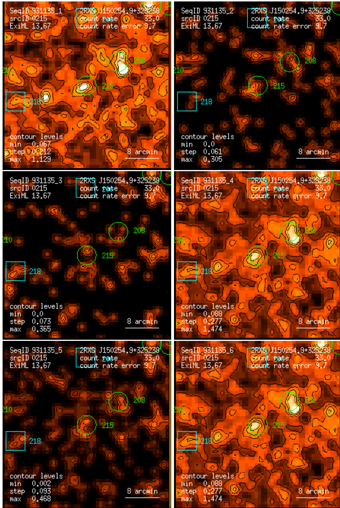
Figure 215: RASS 931135: detection 0215: band rate images, Gaussian filter: (1) PSPC channels 11 – 41, (2) 52 – 90, (3) 91 – 201, (4) 11 – 235, (5) 52 – 201, (6) 11 – 201. Broad band rates in counts/ks. Band rate contour levels in counts/ks/arcmin 2 .
