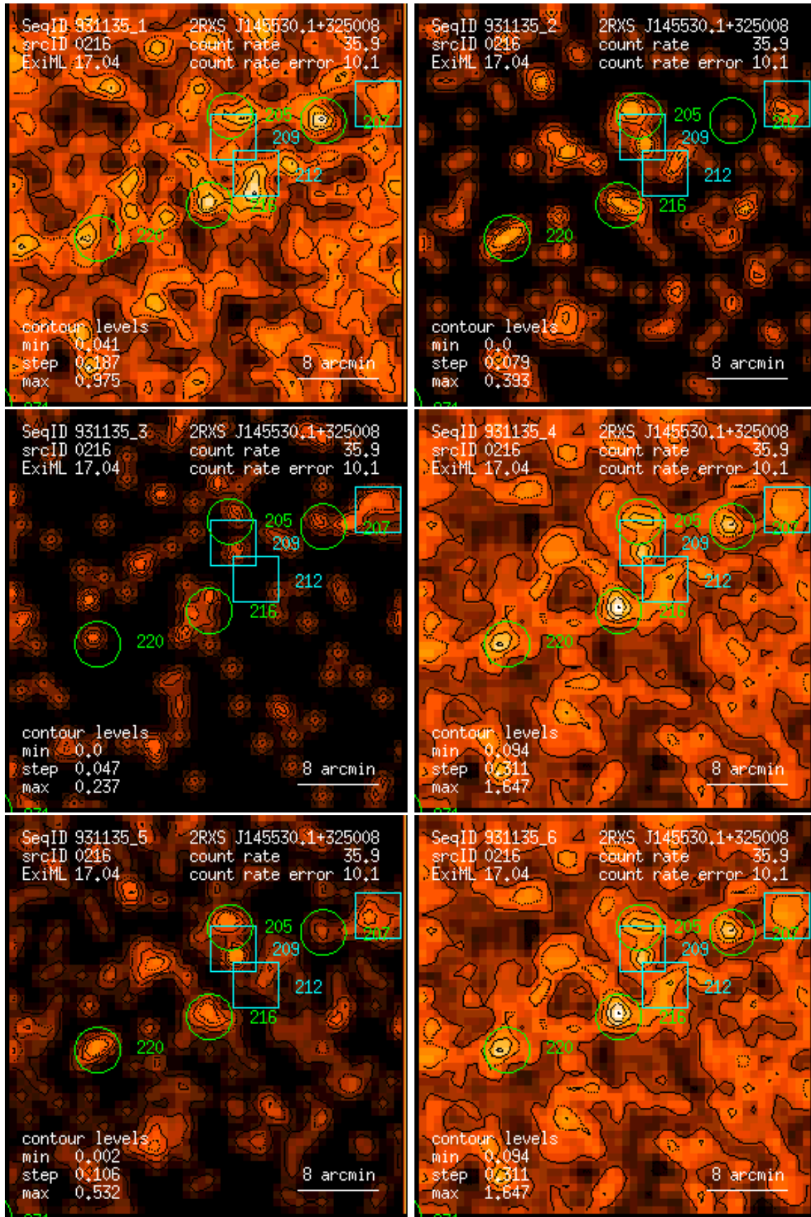
Figure 216: RASS 931135: detection 0216: band rate images, Gaussian filter: (1) PSPC channels 11 – 41, (2) 52 – 90, (3) 91 – 201, (4) 11 – 235, (5) 52 – 201, (6) 11 – 201. Broad band rates in counts/ks. Band rate contour levels in counts/ks/arcmin 2 .
