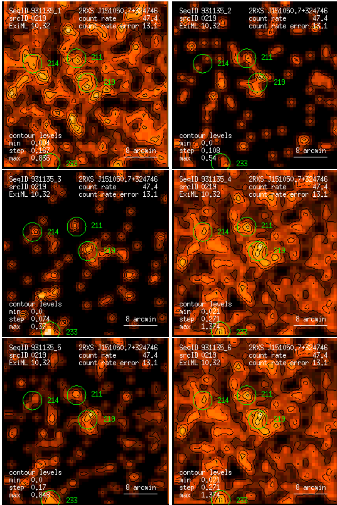
Figure 219: RASS 931135: detection 0219: band rate images, Gaussian filter: (1) PSPC channels 11 – 41, (2) 52 – 90, (3) 91 – 201, (4) 11 – 235, (5) 52 – 201, (6) 11 – 201. Broad band rates in counts/ks. Band rate contour levels in counts/ks/arcmin 2 .
