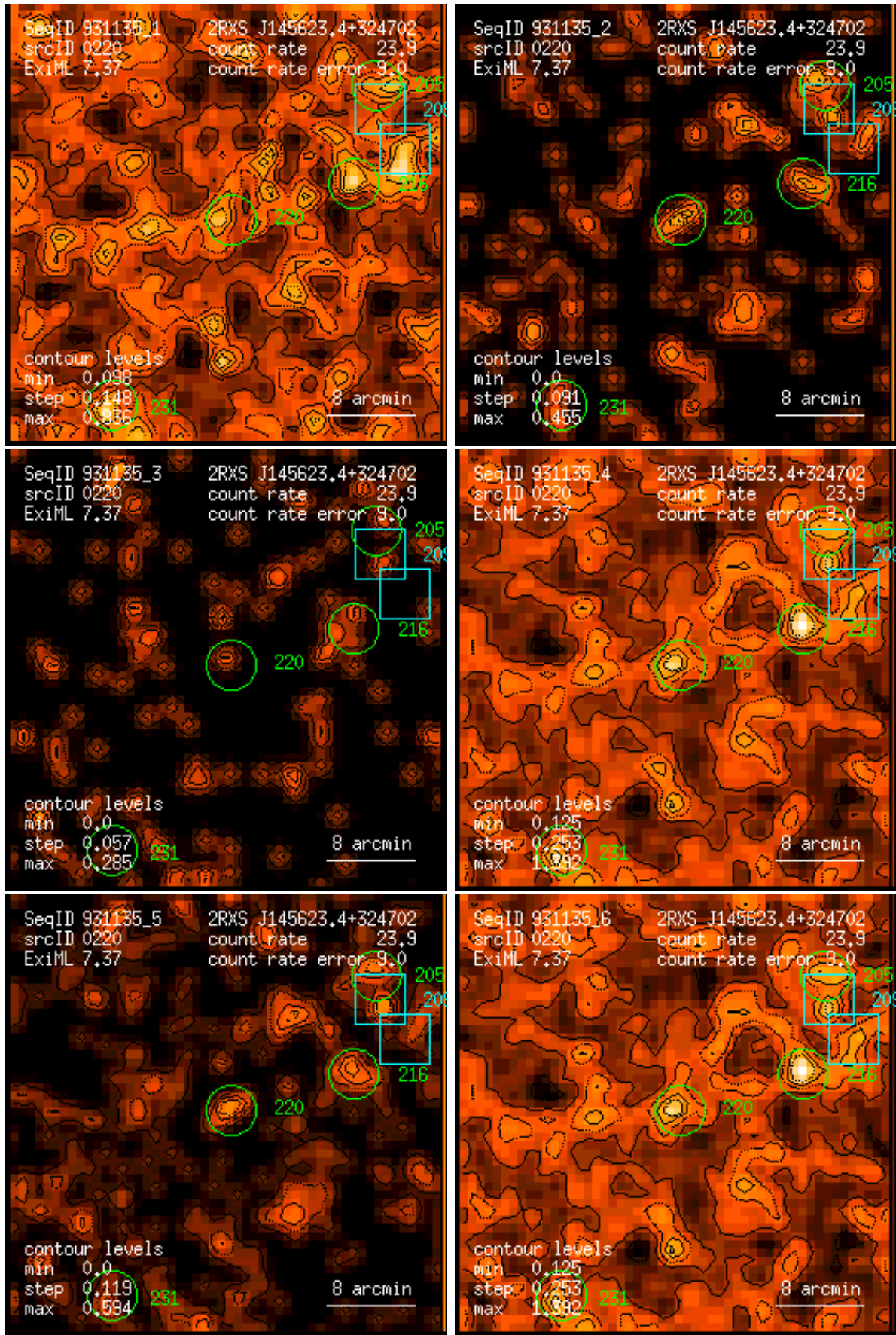
Figure 220: RASS 931135: detection 0220: band rate images, Gaussian filter: (1) PSPC channels 11 – 41, (2) 52 – 90, (3) 91 – 201, (4) 11 – 235, (5) 52 – 201, (6) 11 – 201. Broad band rates in counts/ks. Band rate contour levels in counts/ks/arcmin 2 .
