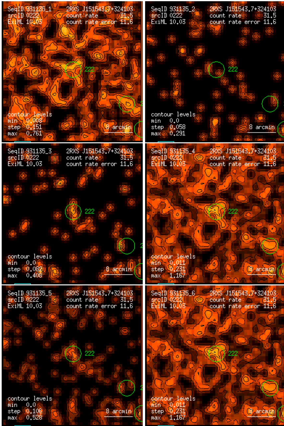
Figure 222: RASS 931135: detection 0222: band rate images, Gaussian filter: (1) PSPC channels 11 – 41, (2) 52 – 90, (3) 91 – 201, (4) 11 – 235, (5) 52 – 201, (6) 11 – 201. Broad band rates in counts/ks. Band rate contour levels in counts/ks/arcmin 2 .
