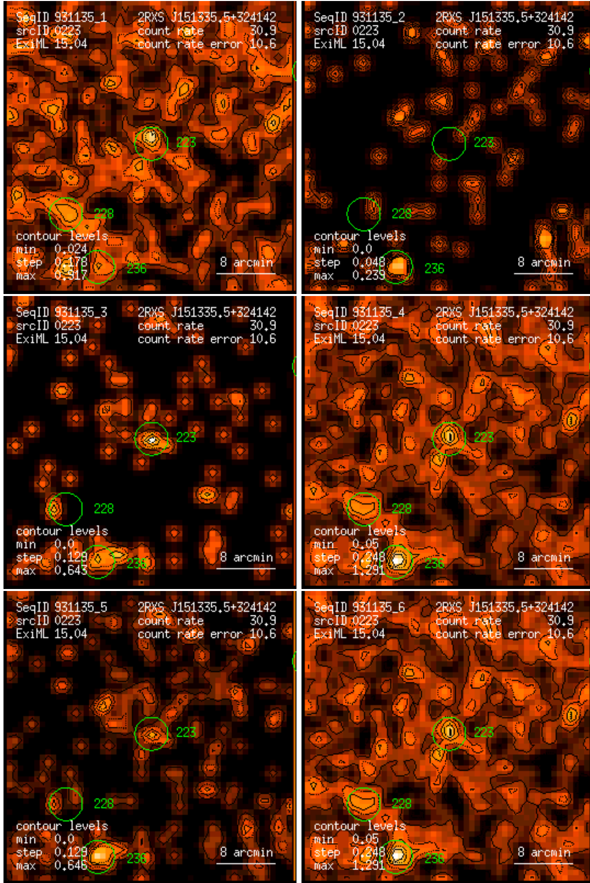
Figure 223: RASS 931135: detection 0223: band rate images, Gaussian filter: (1) PSPC channels 11 – 41, (2) 52 – 90, (3) 91 – 201, (4) 11 – 235, (5) 52 – 201, (6) 11 – 201. Broad band rates in counts/ks. Band rate contour levels in counts/ks/arcmin 2 .
