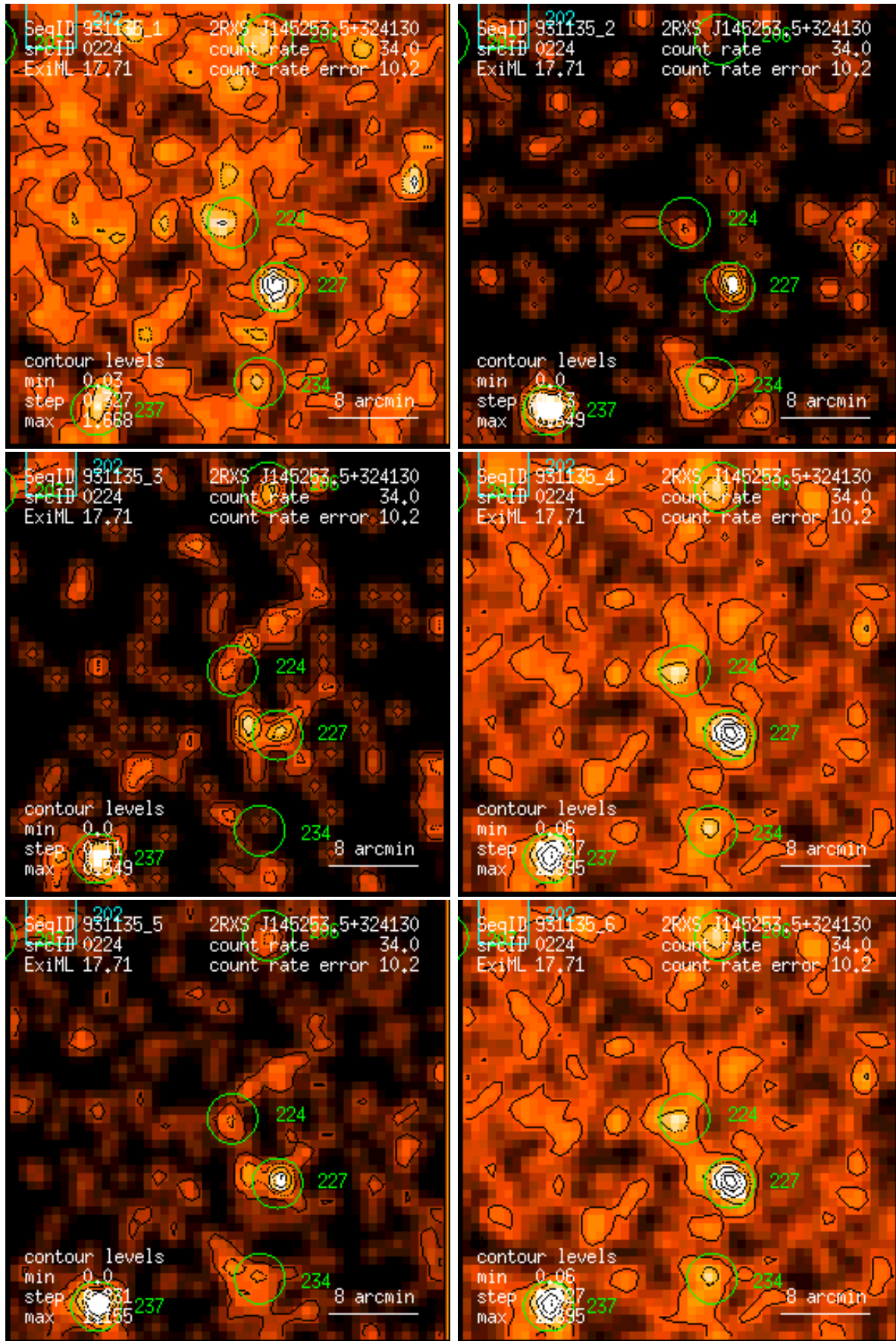
Figure 224: RASS 931135: detection 0224: band rate images, Gaussian filter: (1) PSPC channels 11 – 41, (2) 52 – 90, (3) 91 – 201, (4) 11 – 235, (5) 52 – 201, (6) 11 – 201. Broad band rates in counts/ks. Band rate contour levels in counts/ks/arcmin 2 .
