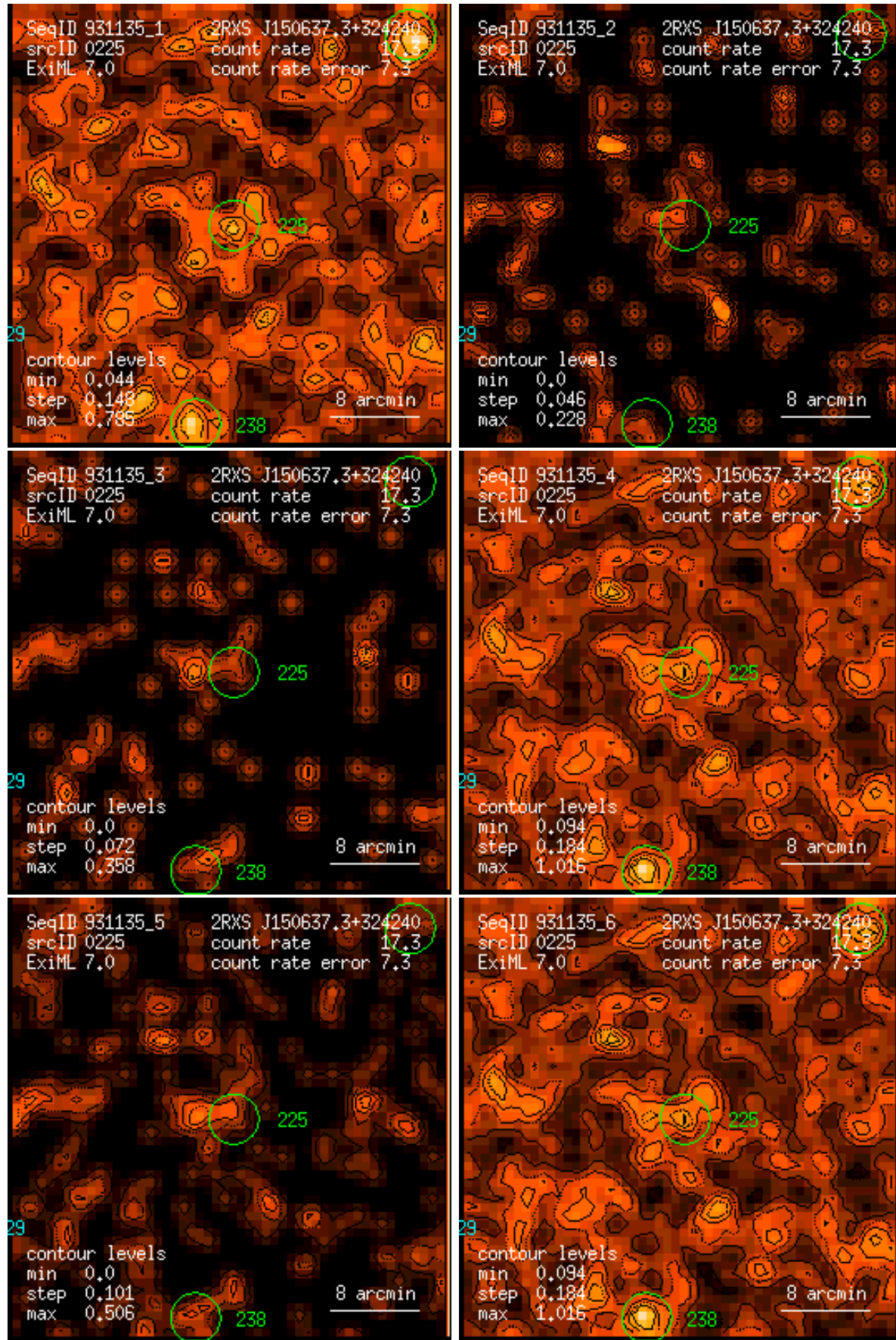
Figure 225: RASS 931135: detection 0225: band rate images, Gaussian filter: (1) PSPC channels 11 – 41, (2) 52 – 90, (3) 91 – 201, (4) 11 – 235, (5) 52 – 201, (6) 11 – 201. Broad band rates in counts/ks. Band rate contour levels in counts/ks/arcmin 2 .
