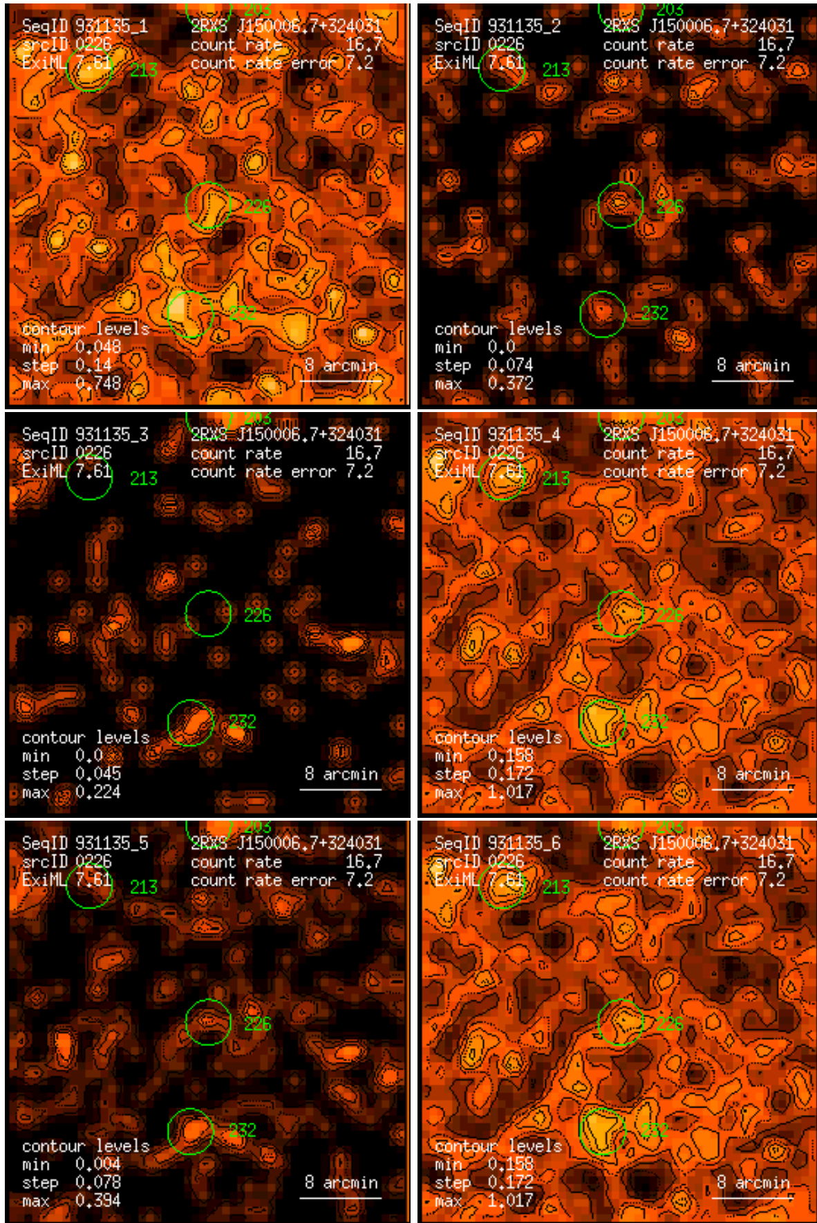
Figure 226: RASS 931135: detection 0226: band rate images, Gaussian filter: (1) PSPC channels 11 – 41, (2) 52 – 90, (3) 91 – 201, (4) 11 – 235, (5) 52 – 201, (6) 11 – 201. Broad band rates in counts/ks. Band rate contour levels in counts/ks/arcmin 2 .
