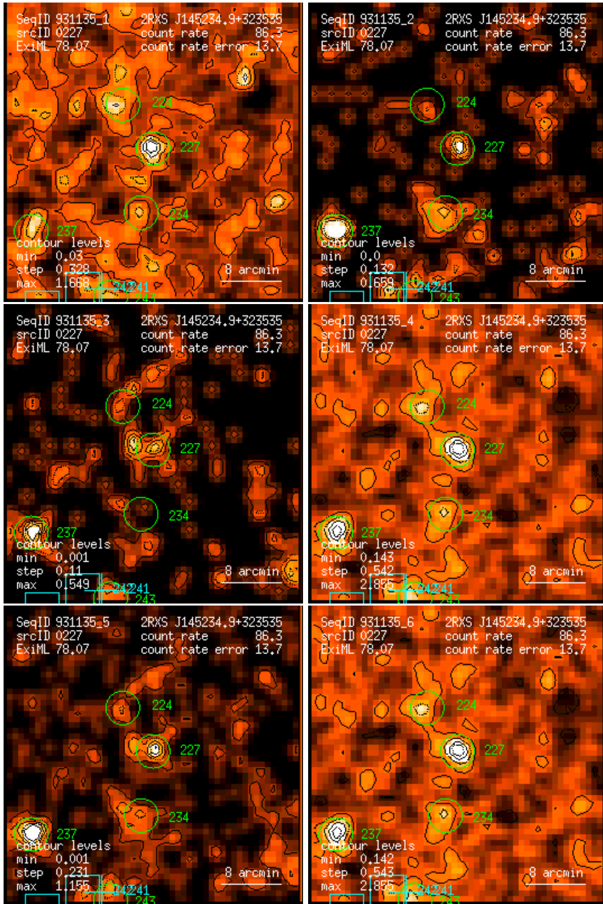
Figure 227: RASS 931135: detection 0227: band rate images, Gaussian filter: (1) PSPC channels 11 – 41, (2) 52 – 90, (3) 91 – 201, (4) 11 – 235, (5) 52 – 201, (6) 11 – 201. Broad band rates in counts/ks. Band rate contour levels in counts/ks/arcmin 2 .
