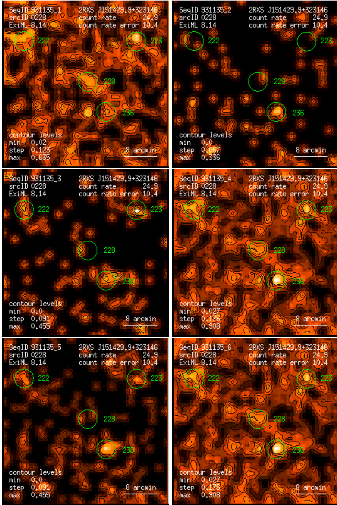
Figure 228: RASS 931135: detection 0228: band rate images, Gaussian filter: (1) PSPC channels 11 – 41, (2) 52 – 90, (3) 91 – 201, (4) 11 – 235, (5) 52 – 201, (6) 11 – 201. Broad band rates in counts/ks. Band rate contour levels in counts/ks/arcmin 2 .
