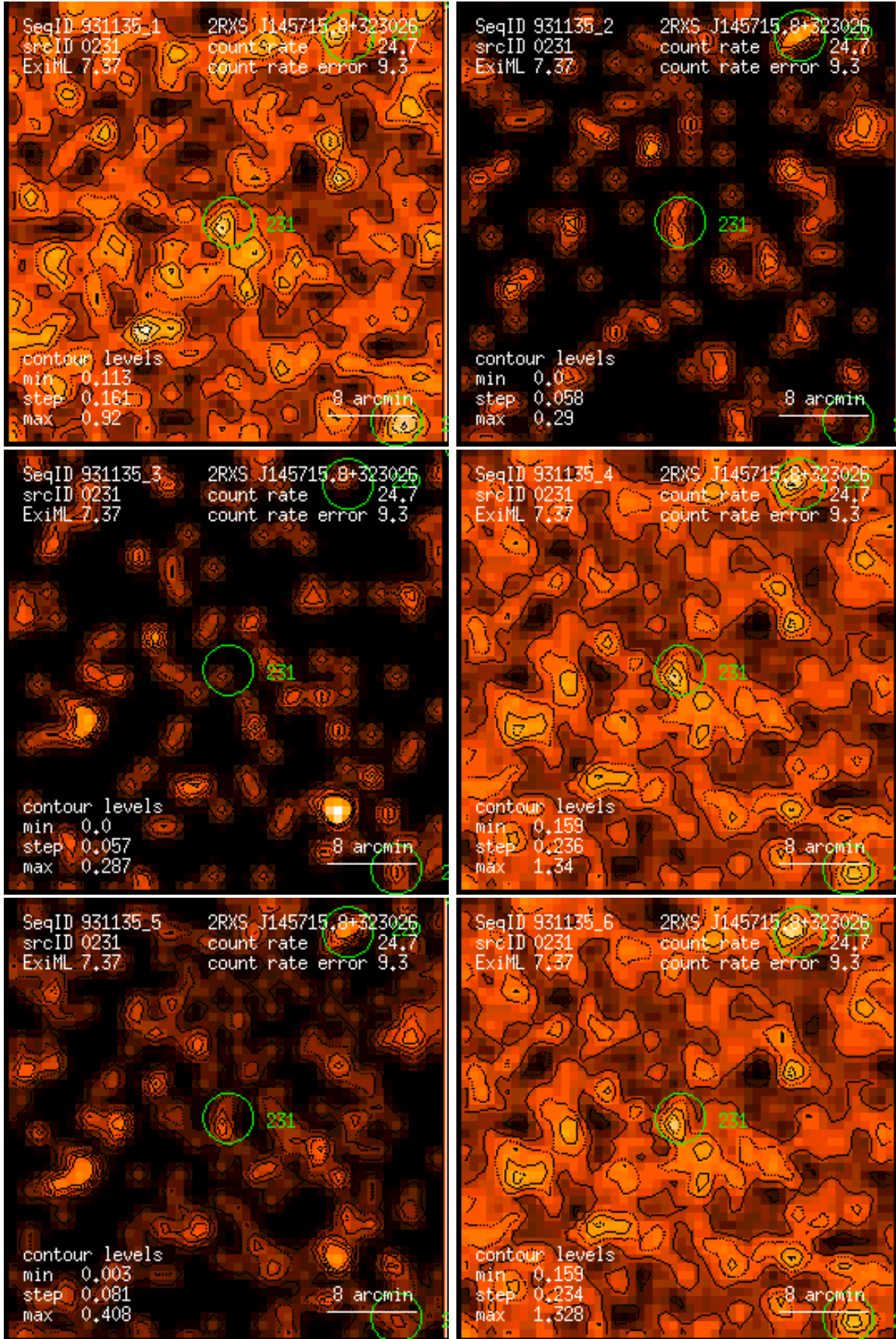
Figure 231: RASS 931135: detection 0231: band rate images, Gaussian filter: (1) PSPC channels 11 – 41, (2) 52 – 90, (3) 91 – 201, (4) 11 – 235, (5) 52 – 201, (6) 11 – 201. Broad band rates in counts/ks. Band rate contour levels in counts/ks/arcmin 2 .
