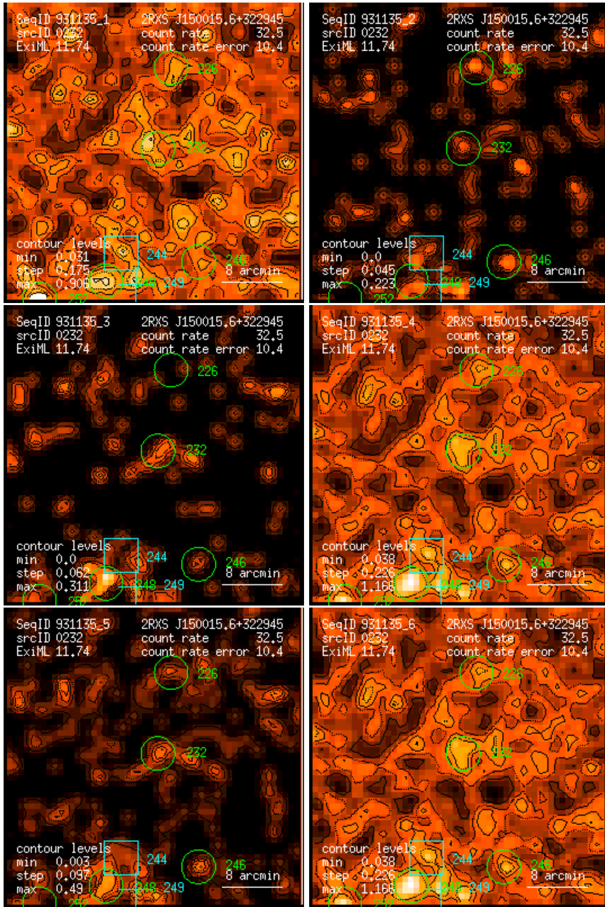
Figure 232: RASS 931135: detection 0232: band rate images, Gaussian filter: (1) PSPC channels 11 – 41, (2) 52 – 90, (3) 91 – 201, (4) 11 – 235, (5) 52 – 201, (6) 11 – 201. Broad band rates in counts/ks. Band rate contour levels in counts/ks/arcmin 2 .
