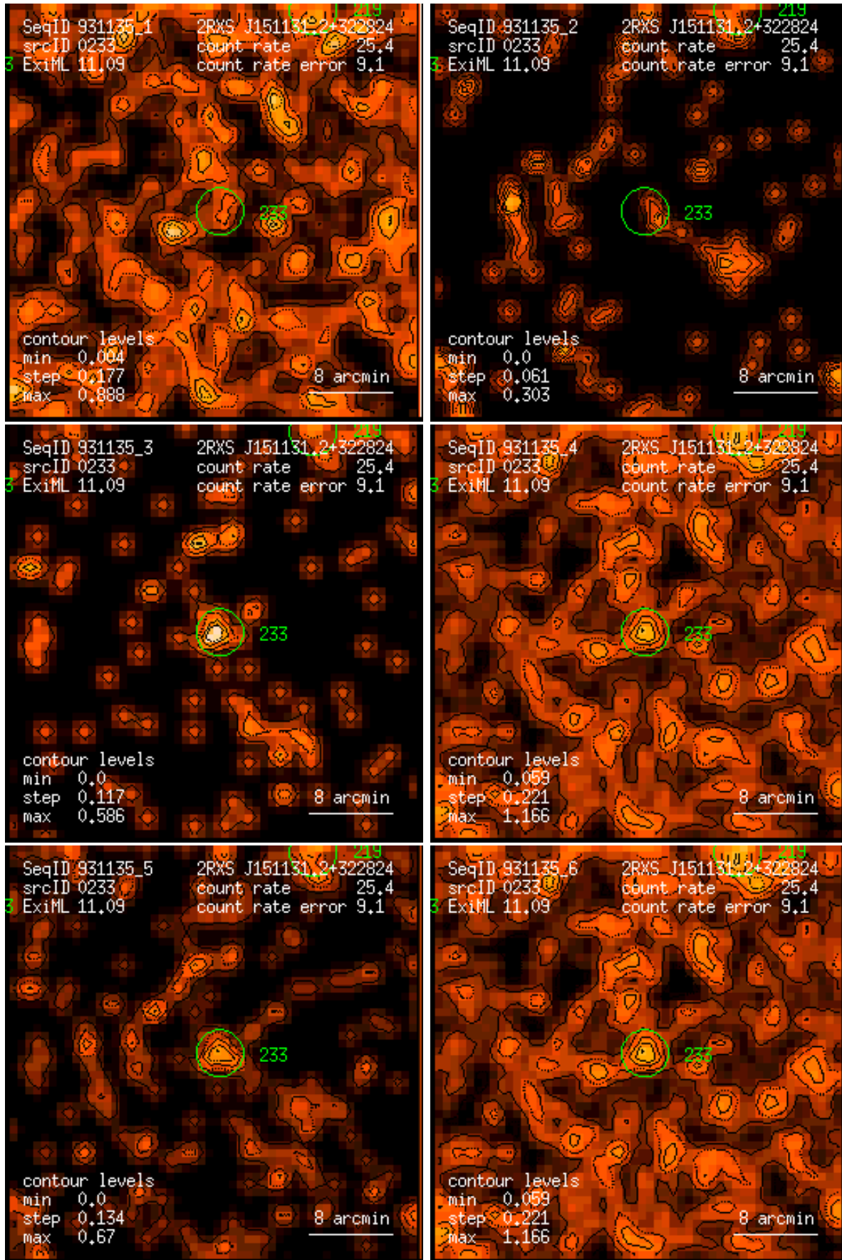
Figure 233: RASS 931135: detection 0233: band rate images, Gaussian filter: (1) PSPC channels 11 – 41, (2) 52 – 90, (3) 91 – 201, (4) 11 – 235, (5) 52 – 201, (6) 11 – 201. Broad band rates in counts/ks. Band rate contour levels in counts/ks/arcmin 2 .
