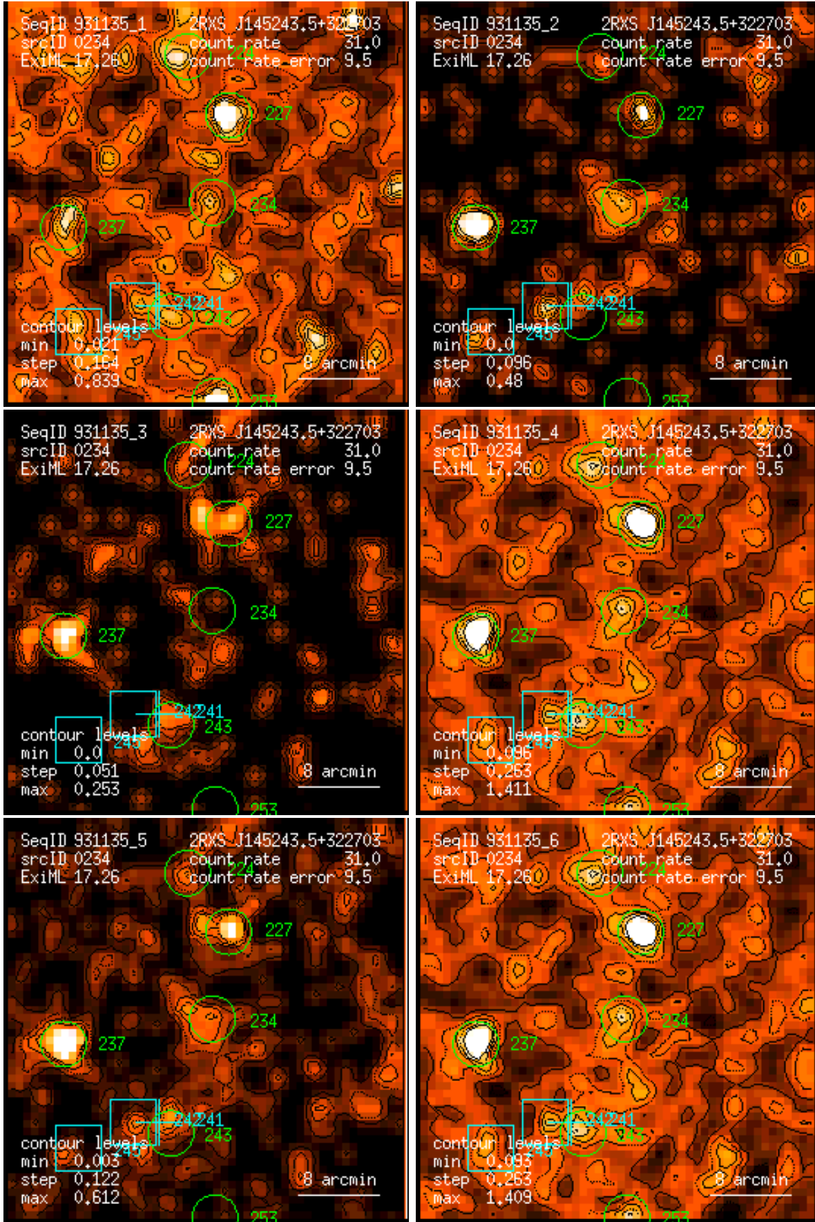
Figure 234: RASS 931135: detection 0234: band rate images, Gaussian filter: (1) PSPC channels 11 – 41, (2) 52 – 90, (3) 91 – 201, (4) 11 – 235, (5) 52 – 201, (6) 11 – 201. Broad band rates in counts/ks. Band rate contour levels in counts/ks/arcmin 2 .
