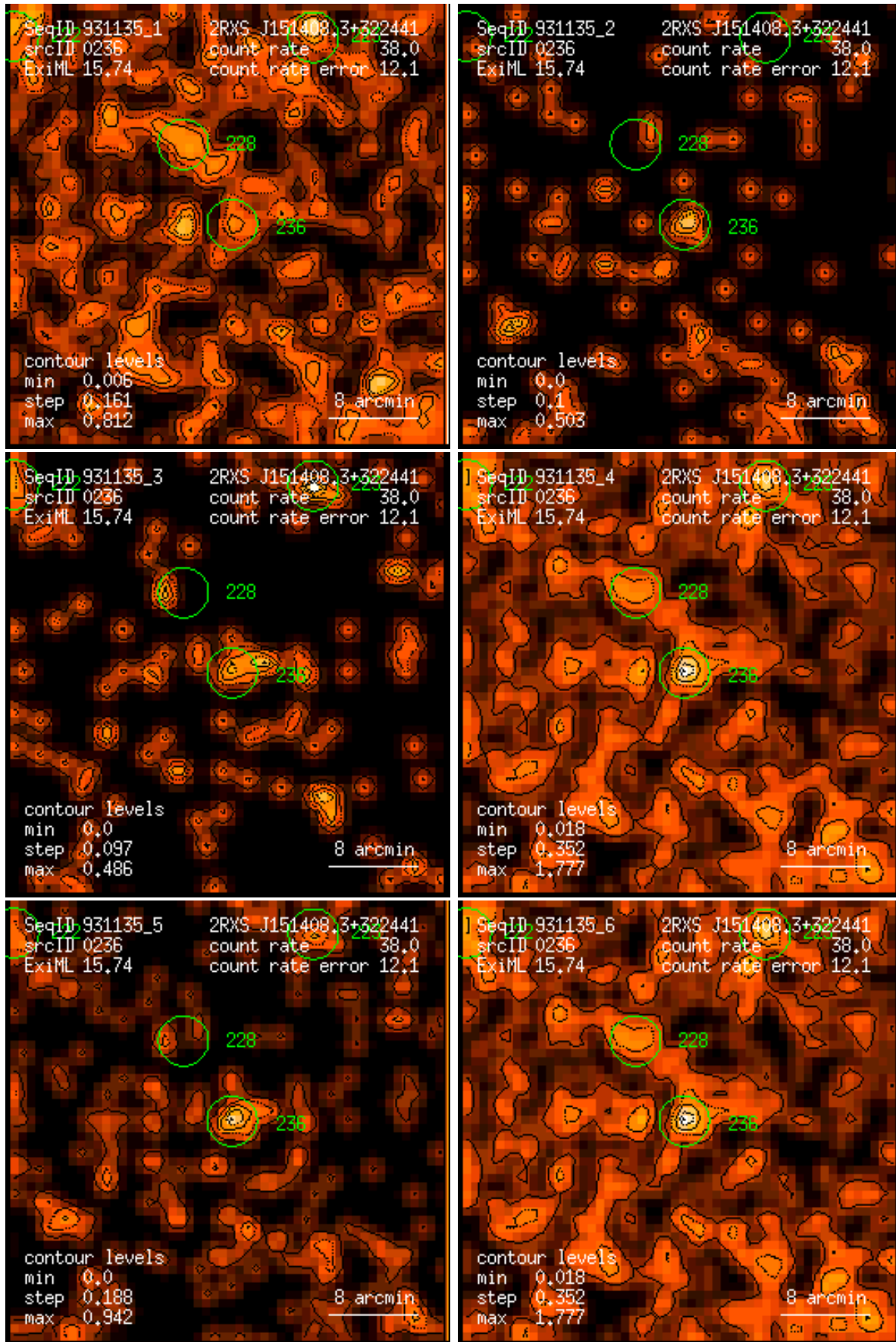
Figure 236: RASS 931135: detection 0236: band rate images, Gaussian filter: (1) PSPC channels 11 – 41, (2) 52 – 90, (3) 91 – 201, (4) 11 – 235, (5) 52 – 201, (6) 11 – 201. Broad band rates in counts/ks. Band rate contour levels in counts/ks/arcmin 2 .
