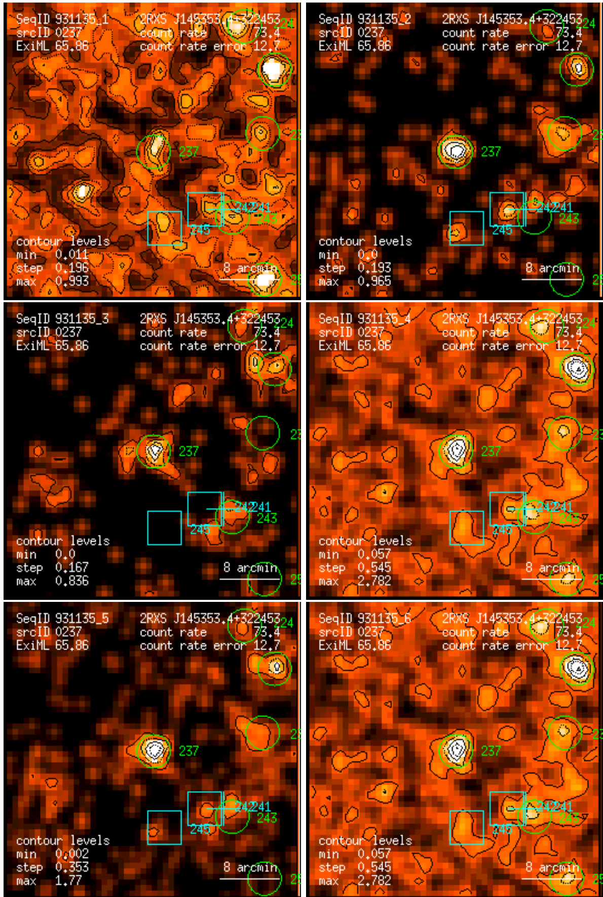
Figure 237: RASS 931135: detection 0237: band rate images, Gaussian filter: (1) PSPC channels 11 – 41, (2) 52 – 90, (3) 91 – 201, (4) 11 – 235, (5) 52 – 201, (6) 11 – 201. Broad band rates in counts/ks. Band rate contour levels in counts/ks/arcmin 2 .
