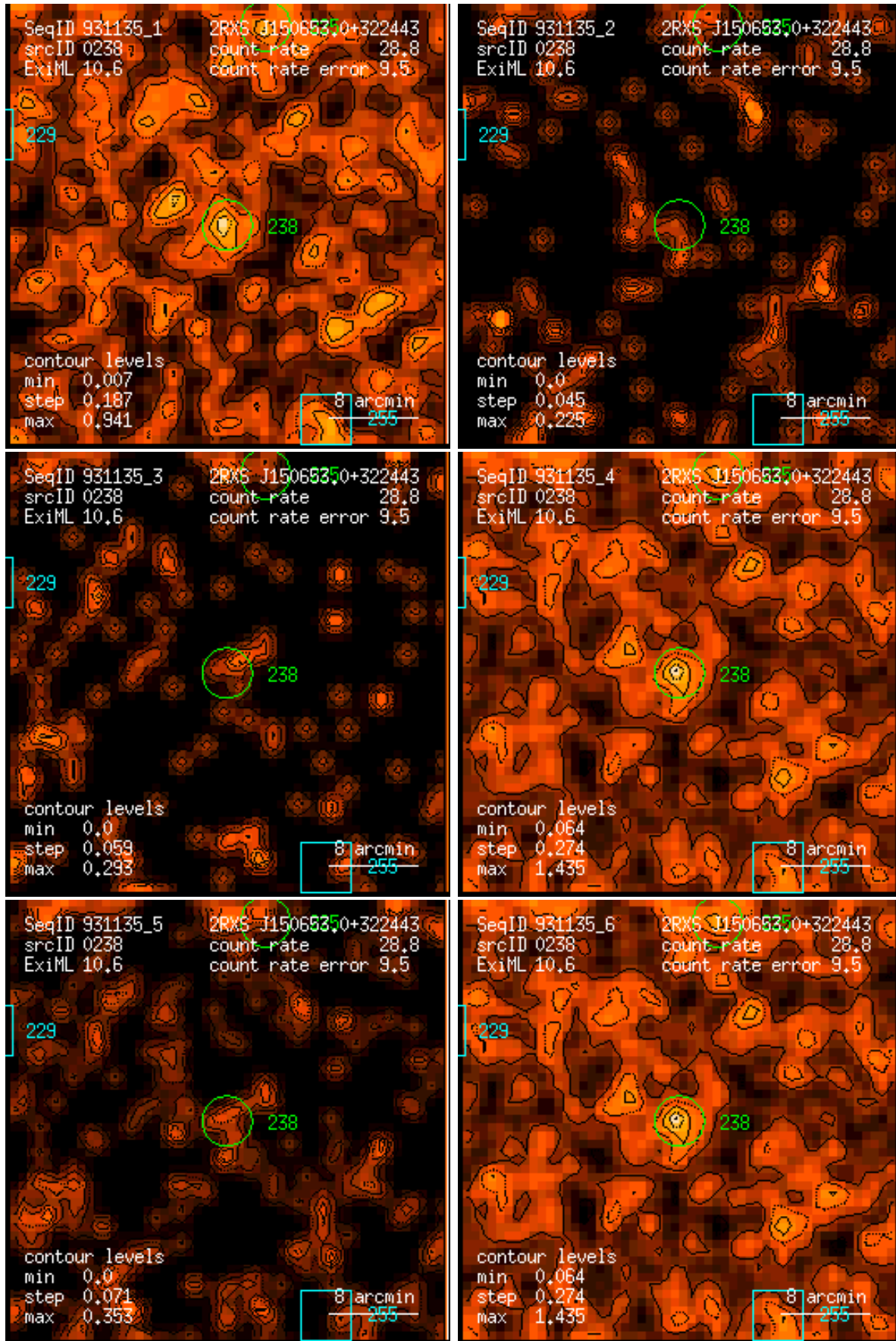
Figure 238: RASS 931135: detection 0238: band rate images, Gaussian filter: (1) PSPC channels 11 – 41, (2) 52 – 90, (3) 91 – 201, (4) 11 – 235, (5) 52 – 201, (6) 11 – 201. Broad band rates in counts/ks. Band rate contour levels in counts/ks/arcmin 2 .
