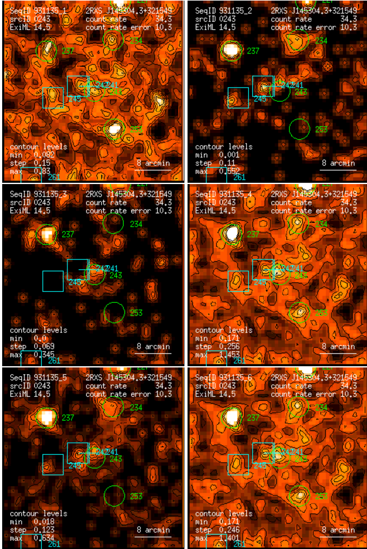
Figure 243: RASS 931135: detection 0243: band rate images, Gaussian filter: (1) PSPC channels 11 – 41, (2) 52 – 90, (3) 91 – 201, (4) 11 – 235, (5) 52 – 201, (6) 11 – 201. Broad band rates in counts/ks. Band rate contour levels in counts/ks/arcmin 2 .
