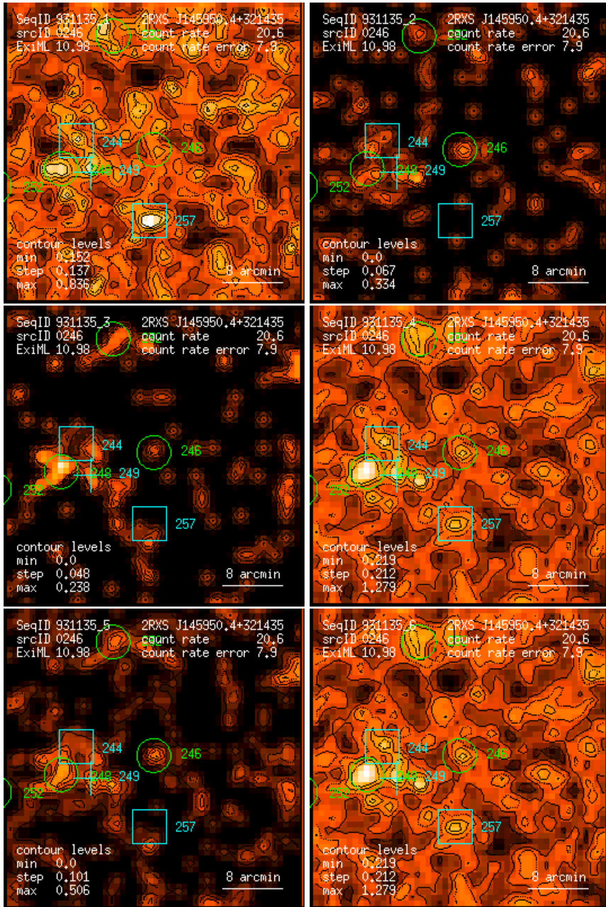
Figure 246: RASS 931135: detection 0246: band rate images, Gaussian filter: (1) PSPC channels 11 – 41, (2) 52 – 90, (3) 91 – 201, (4) 11 – 235, (5) 52 – 201, (6) 11 – 201. Broad band rates in counts/ks. Band rate contour levels in counts/ks/arcmin 2 .
