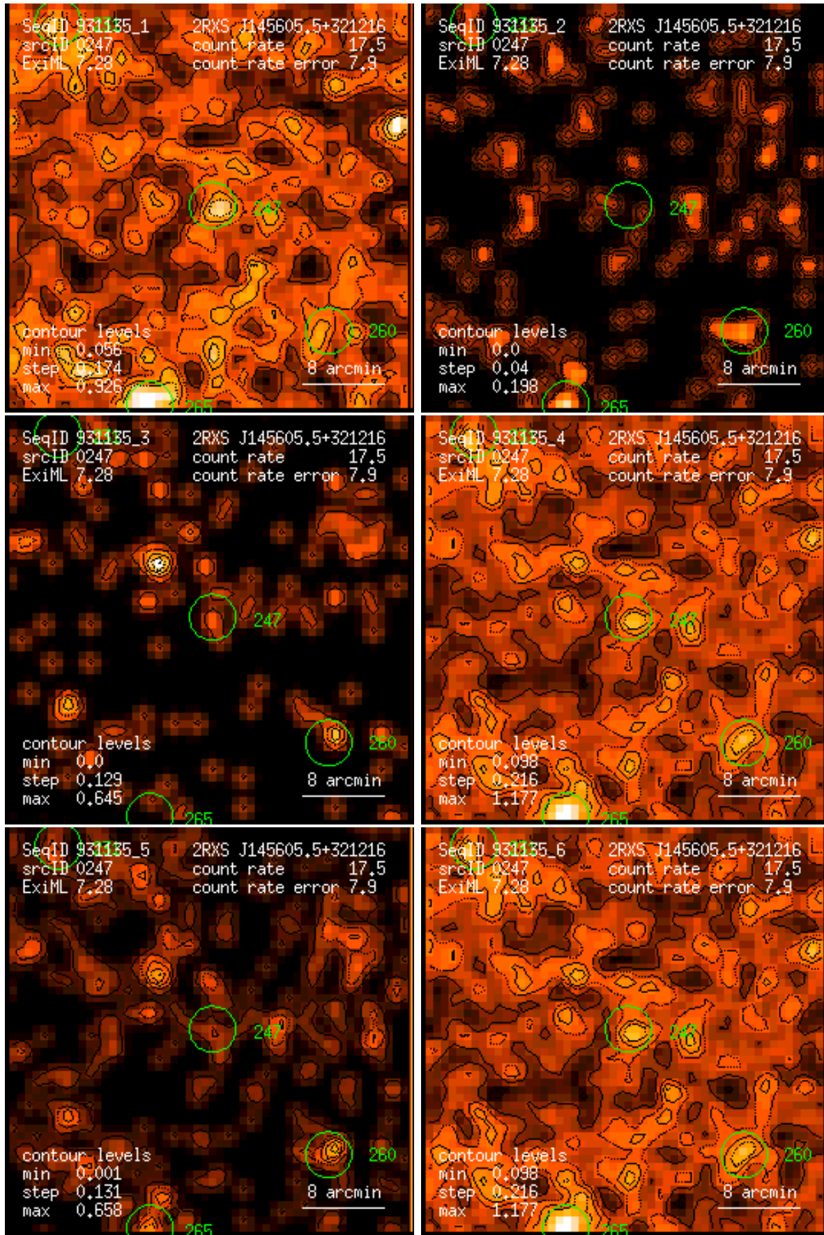
Figure 247: RASS 931135: detection 0247: band rate images, Gaussian filter: (1) PSPC channels 11 – 41, (2) 52 – 90, (3) 91 – 201, (4) 11 – 235, (5) 52 – 201, (6) 11 – 201. Broad band rates in counts/ks. Band rate contour levels in counts/ks/arcmin 2 .
