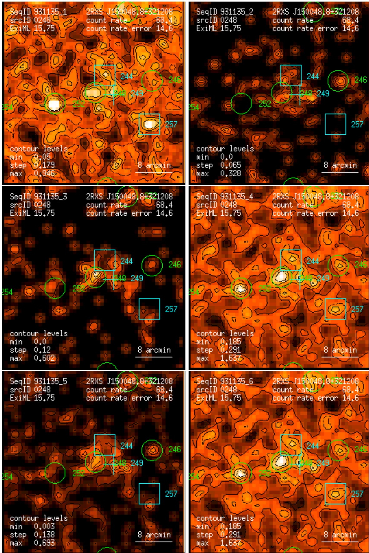
Figure 248: RASS 931135: detection 0248: band rate images, Gaussian filter: (1) PSPC channels 11 – 41, (2) 52 – 90, (3) 91 – 201, (4) 11 – 235, (5) 52 – 201, (6) 11 – 201. Broad band rates in counts/ks. Band rate contour levels in counts/ks/arcmin 2 .
