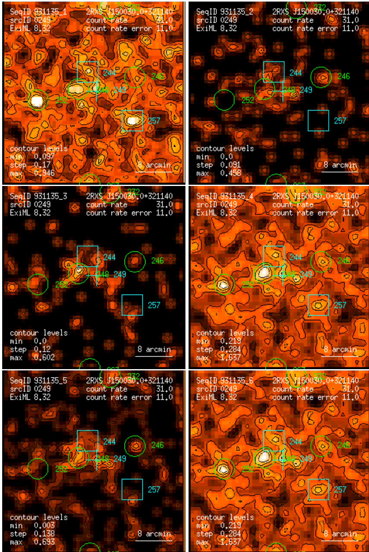
Figure 249: RASS 931135: detection 0249: band rate images, Gaussian filter: (1) PSPC channels 11 – 41, (2) 52 – 90, (3) 91 – 201, (4) 11 – 235, (5) 52 – 201, (6) 11 – 201. Broad band rates in counts/ks. Band rate contour levels in counts/ks/arcmin 2 .
