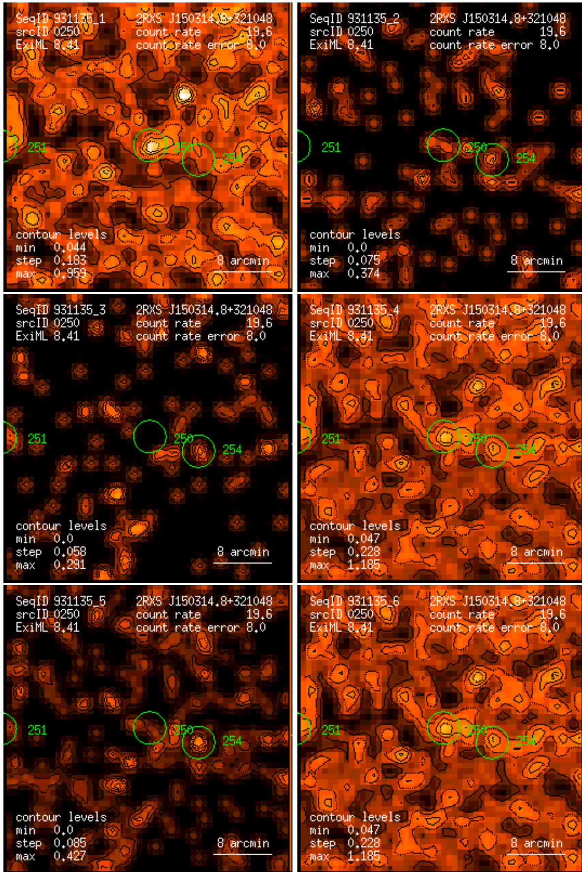
Figure 250: RASS 931135: detection 0250: band rate images, Gaussian filter: (1) PSPC channels 11 – 41, (2) 52 – 90, (3) 91 – 201, (4) 11 – 235, (5) 52 – 201, (6) 11 – 201. Broad band rates in counts/ks. Band rate contour levels in counts/ks/arcmin 2 .
