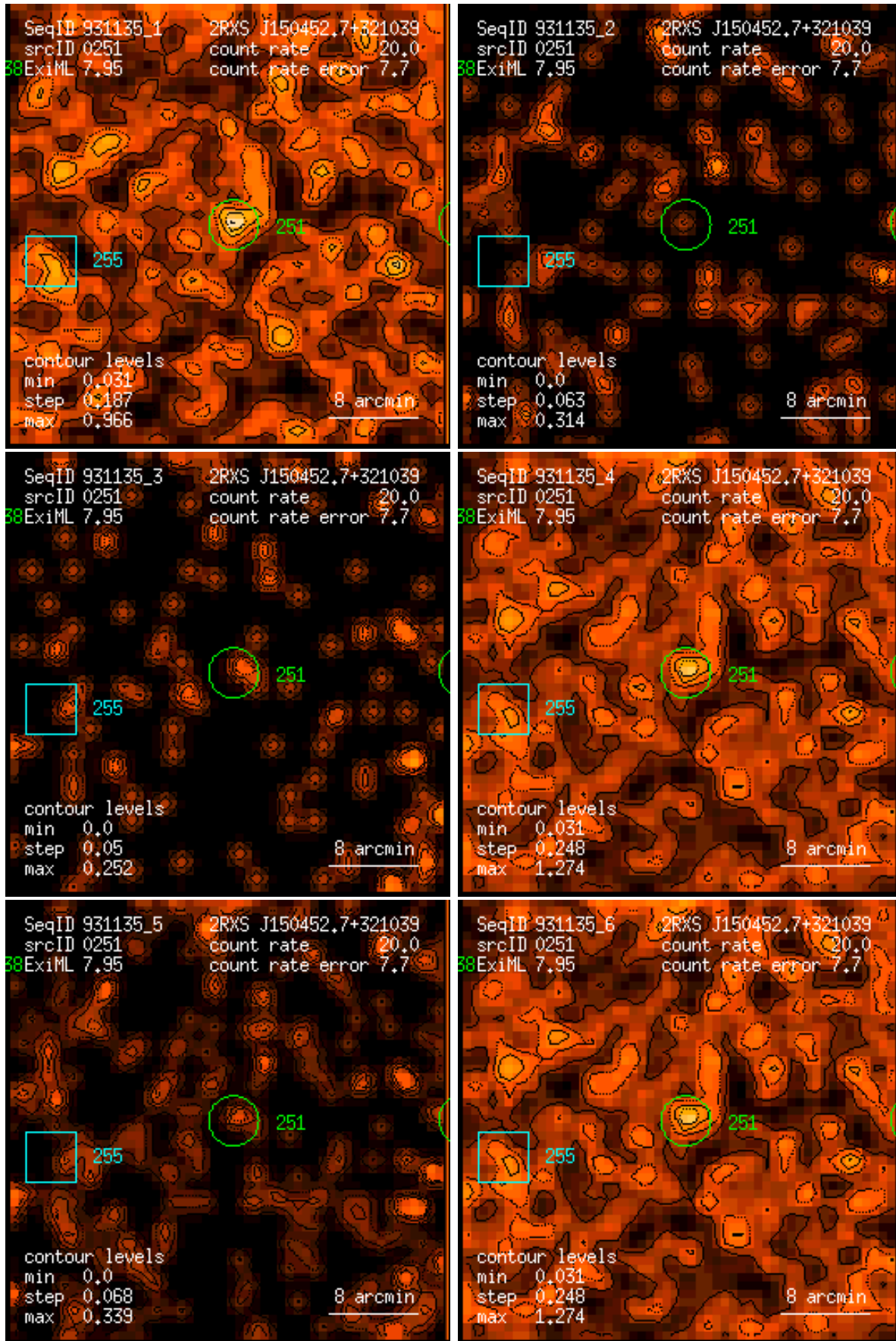
Figure 251: RASS 931135: detection 0251: band rate images, Gaussian filter: (1) PSPC channels 11 – 41, (2) 52 – 90, (3) 91 – 201, (4) 11 – 235, (5) 52 – 201, (6) 11 – 201. Broad band rates in counts/ks. Band rate contour levels in counts/ks/arcmin 2 .
