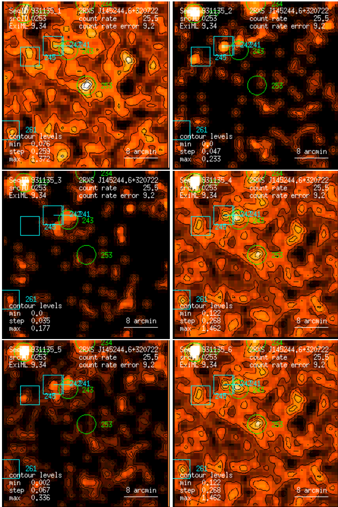
Figure 253: RASS 931135: detection 0253: band rate images, Gaussian filter: (1) PSPC channels 11 – 41, (2) 52 – 90, (3) 91 – 201, (4) 11 – 235, (5) 52 – 201, (6) 11 – 201. Broad band rates in counts/ks. Band rate contour levels in counts/ks/arcmin 2 .
