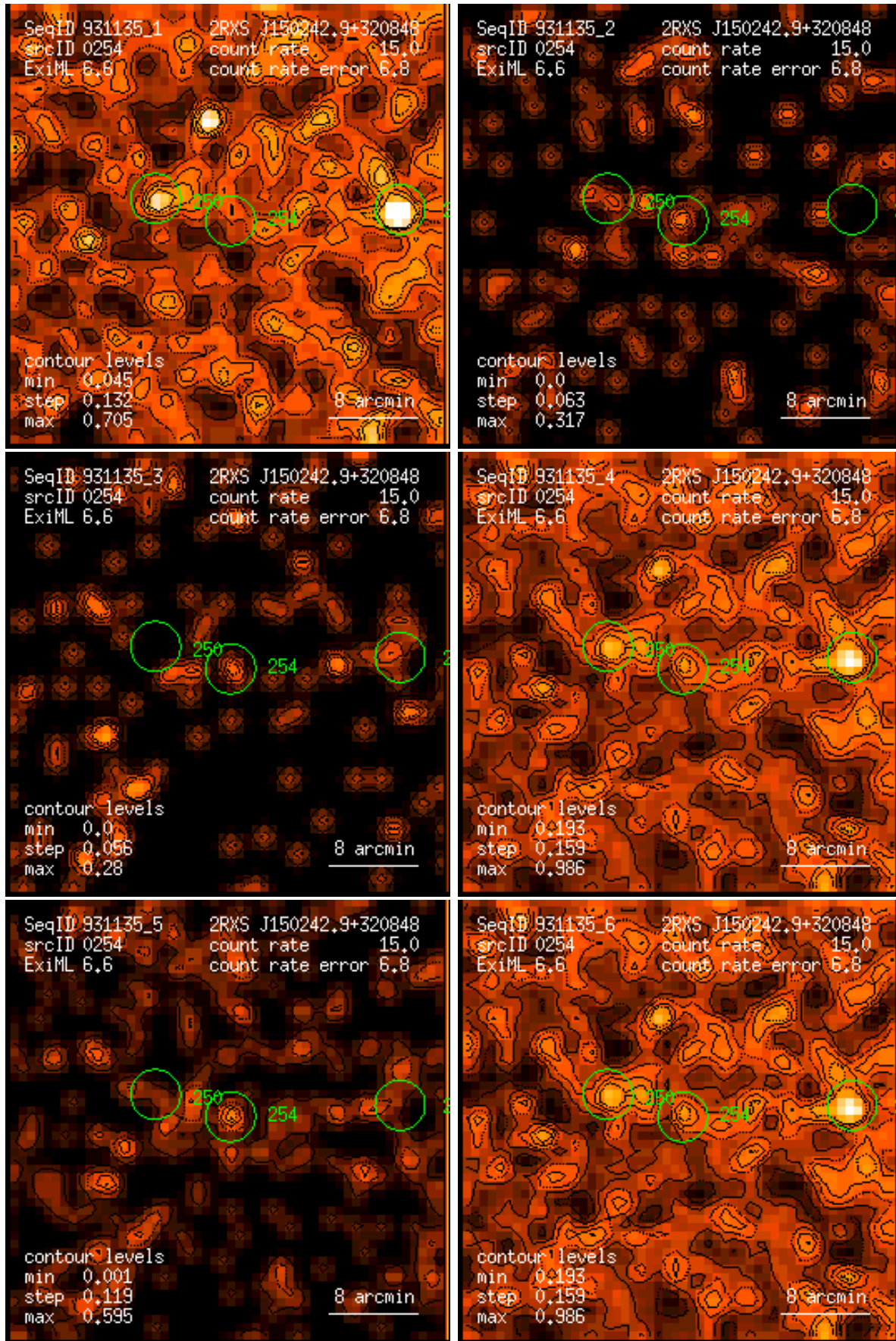
Figure 254: RASS 931135: detection 0254: band rate images, Gaussian filter: (1) PSPC channels 11 – 41, (2) 52 – 90, (3) 91 – 201, (4) 11 – 235, (5) 52 – 201, (6) 11 – 201. Broad band rates in counts/ks. Band rate contour levels in counts/ks/arcmin 2 .
