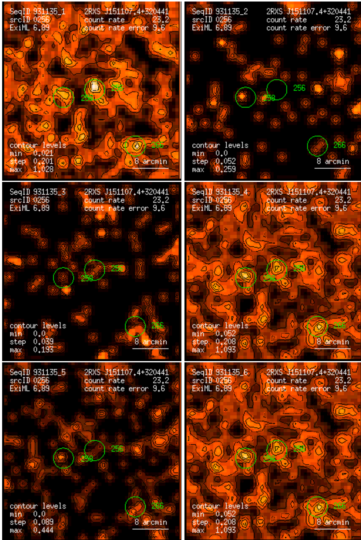
Figure 256: RASS 931135: detection 0256: band rate images, Gaussian filter: (1) PSPC channels 11 – 41, (2) 52 – 90, (3) 91 – 201, (4) 11 – 235, (5) 52 – 201, (6) 11 – 201. Broad band rates in counts/ks. Band rate contour levels in counts/ks/arcmin 2 .
