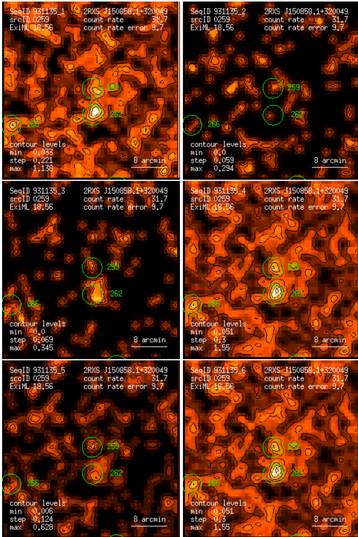
Figure 259: RASS 931135: detection 0259: band rate images, Gaussian filter: (1) PSPC channels 11 – 41, (2) 52 – 90, (3) 91 – 201, (4) 11 – 235, (5) 52 – 201, (6) 11 – 201. Broad band rates in counts/ks. Band rate contour levels in counts/ks/arcmin 2 .
