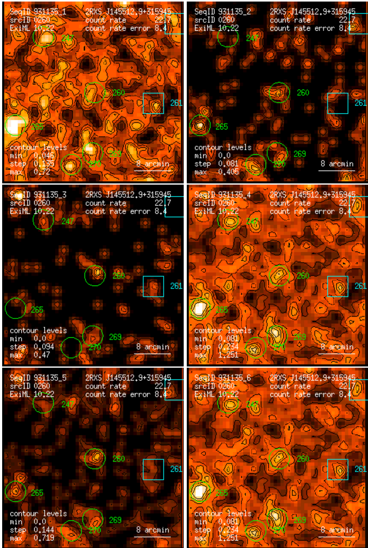
Figure 260: RASS 931135: detection 0260: band rate images, Gaussian filter: (1) PSPC channels 11 – 41, (2) 52 – 90, (3) 91 – 201, (4) 11 – 235, (5) 52 – 201, (6) 11 – 201. Broad band rates in counts/ks. Band rate contour levels in counts/ks/arcmin 2 .
