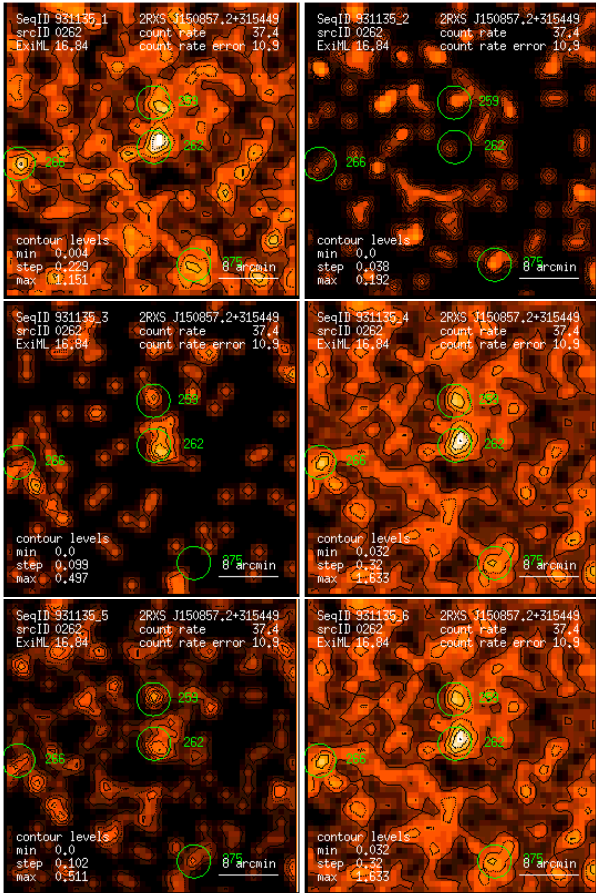
Figure 262: RASS 931135: detection 0262: band rate images, Gaussian filter: (1) PSPC channels 11 – 41, (2) 52 – 90, (3) 91 – 201, (4) 11 – 235, (5) 52 – 201, (6) 11 – 201. Broad band rates in counts/ks. Band rate contour levels in counts/ks/arcmin 2 .
