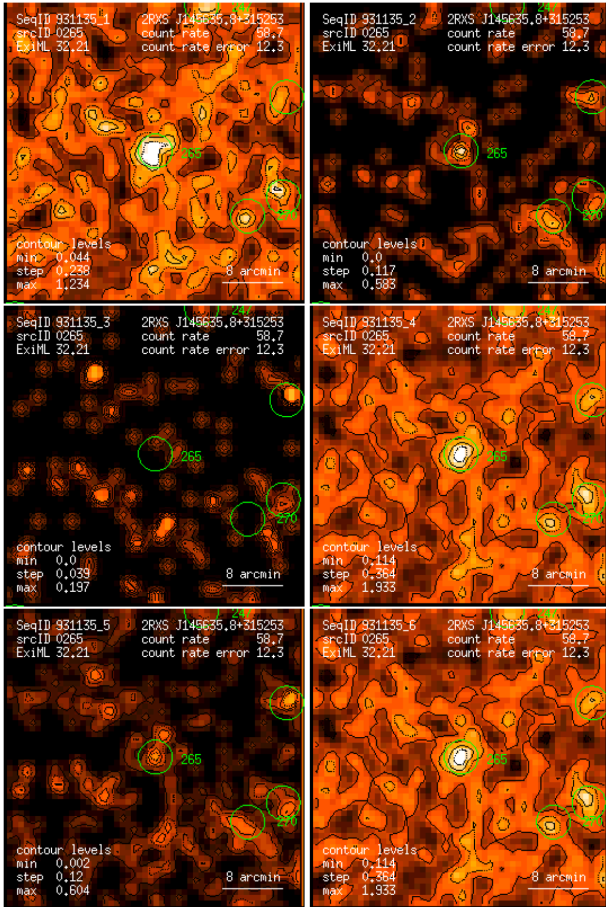
Figure 265: RASS 931135: detection 0265: band rate images, Gaussian filter: (1) PSPC channels 11 – 41, (2) 52 – 90, (3) 91 – 201, (4) 11 – 235, (5) 52 – 201, (6) 11 – 201. Broad band rates in counts/ks. Band rate contour levels in counts/ks/arcmin 2 .
