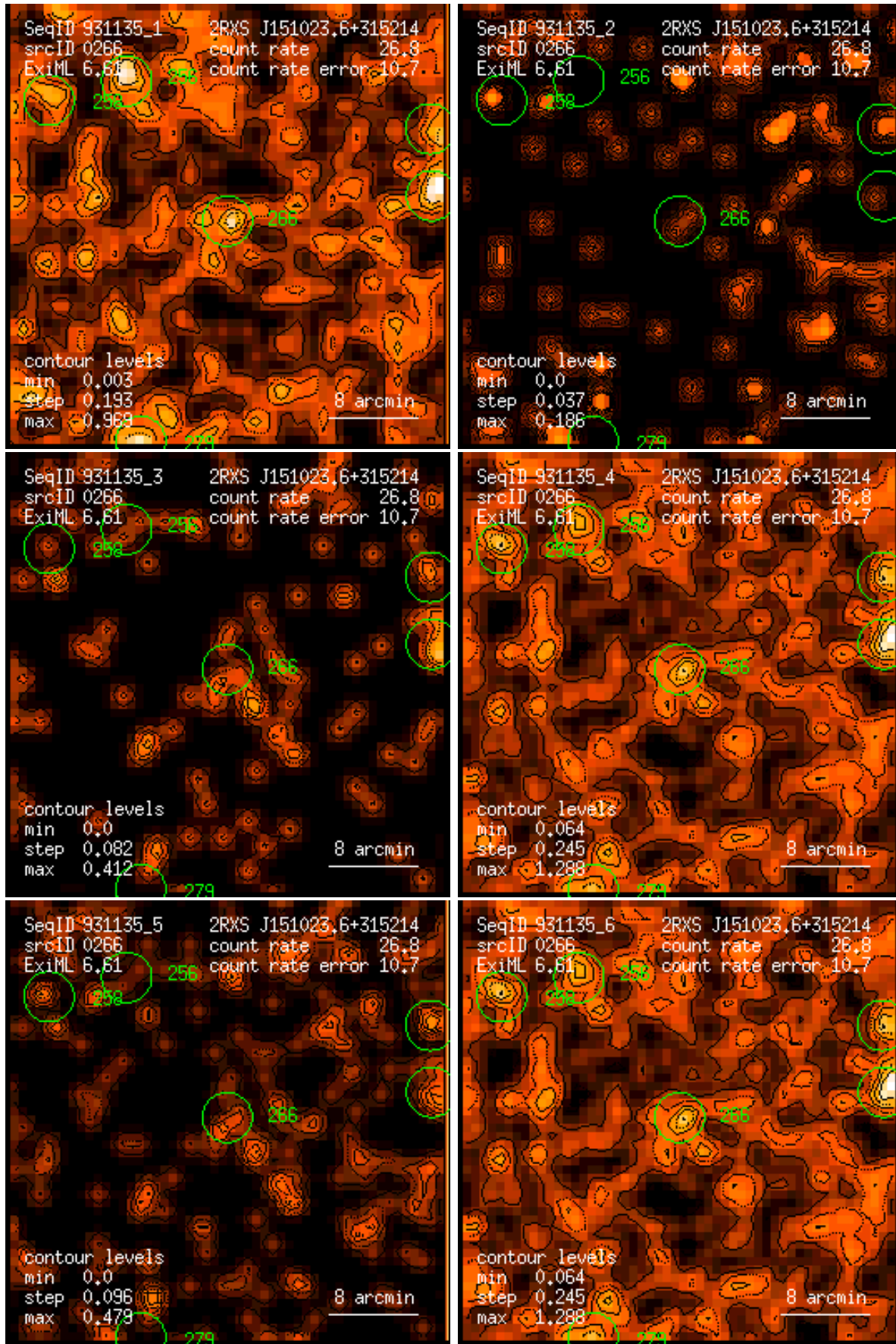
Figure 266: RASS 931135: detection 0266: band rate images, Gaussian filter: (1) PSPC channels 11 – 41, (2) 52 – 90, (3) 91 – 201, (4) 11 – 235, (5) 52 – 201, (6) 11 – 201. Broad band rates in counts/ks. Band rate contour levels in counts/ks/arcmin 2 .
