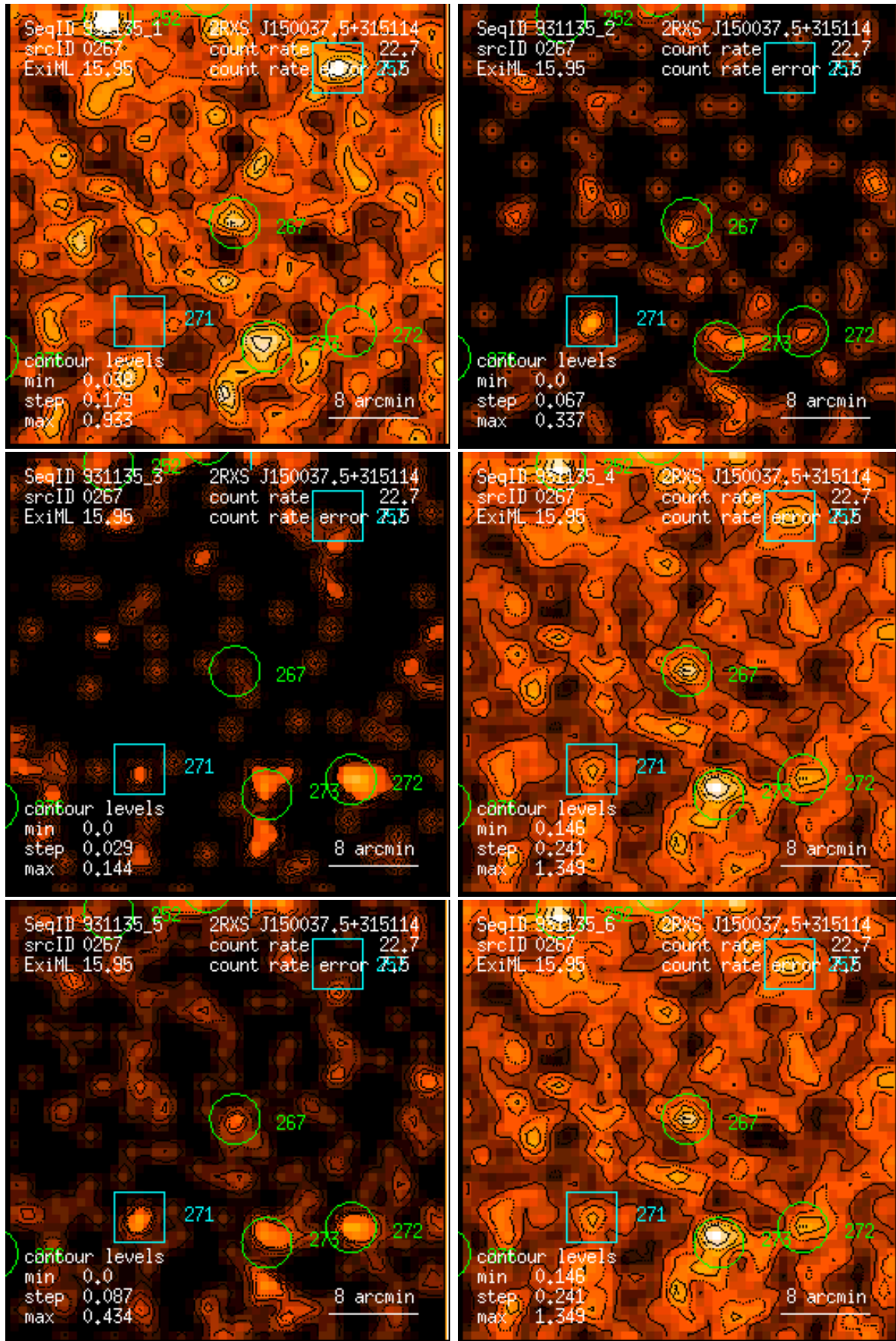
Figure 267: RASS 931135: detection 0267: band rate images, Gaussian filter: (1) PSPC channels 11 – 41, (2) 52 – 90, (3) 91 – 201, (4) 11 – 235, (5) 52 – 201, (6) 11 – 201. Broad band rates in counts/ks. Band rate contour levels in counts/ks/arcmin 2 .
