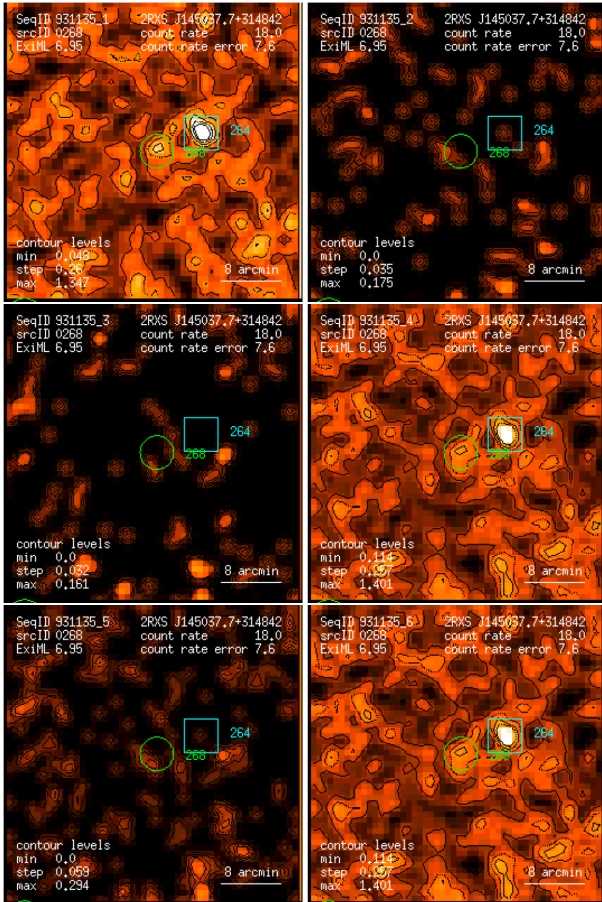
Figure 268: RASS 931135: detection 0268: band rate images, Gaussian filter: (1) PSPC channels 11 – 41, (2) 52 – 90, (3) 91 – 201, (4) 11 – 235, (5) 52 – 201, (6) 11 – 201. Broad band rates in counts/ks. Band rate contour levels in counts/ks/arcmin 2 .
